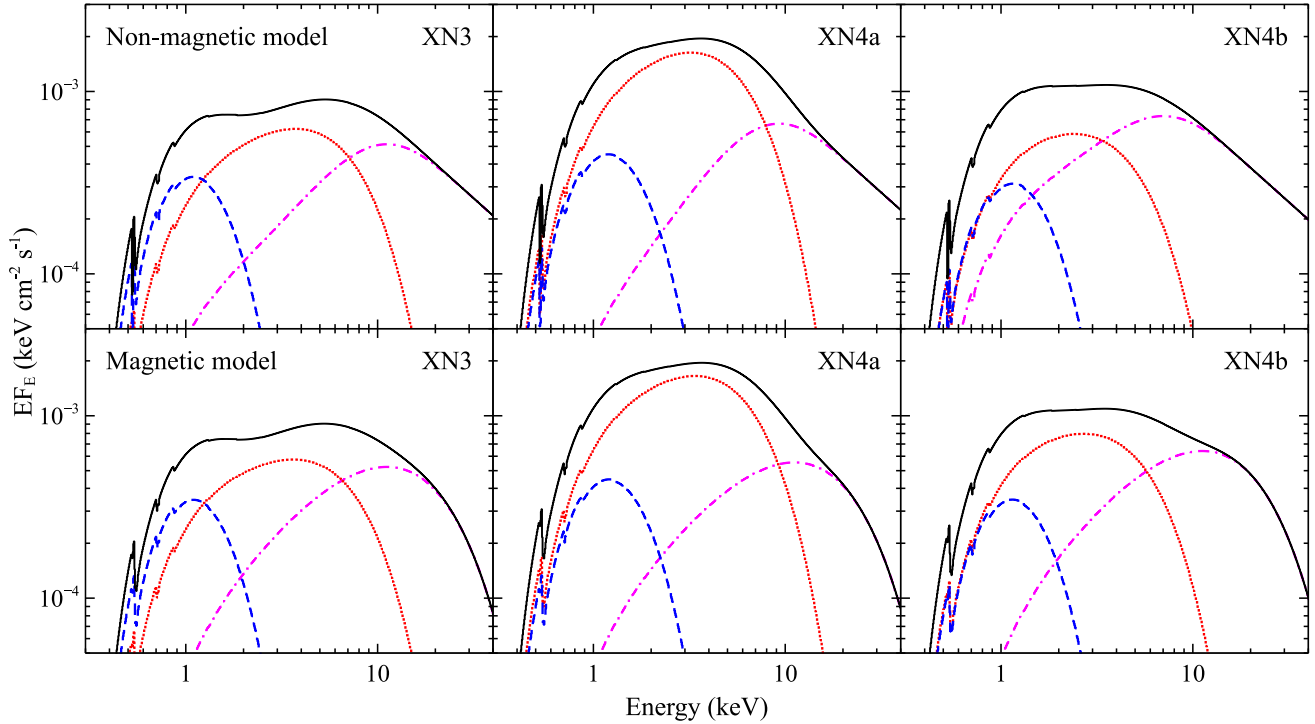
Figure 5. Example model fits for the non-magnetic accretor ( top panels ) and the magnetic accretor ( bottom panels ) models. We show the fits for epochs XN3 (representing the low-flux end of the broadband spectra; left panels ), XN4a (the high-flux end of the broadband spectra, middle panels ), and XN4b (one of the intermediate flux spectra; right panels ). For both models, the total model is shown in solid black, the cooler DISKBB and the hotter DISKBB components are shown in dashed blue and dotted red, respectively (in the black hole case, the DISKBB component is shown as it would appear prior to the application of the SIMPL convolution model), and the highest energy component (either SIMPL or CUTOFFPL) is shown in dash-dot magenta. For the non-magnetic model, the contribution from SIMPL has been calculated by subtracting the unmodified DISKBB component from the combined SIMPL \otimes DISKBB contribution to the fit.
