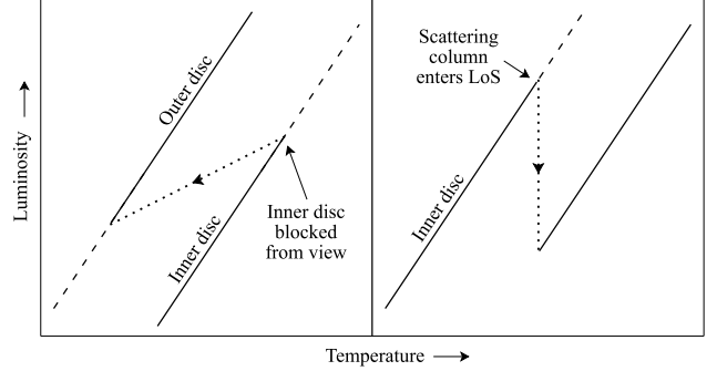
Figure 7. Toy models for the luminosity–temperature plane for the scenarios in which the inner disc is suddenly fully obscured by the outer disc/wind (left panel; discussed in Section 4.2) and in which the emission from the inner disc is scattered by a highly ionised wind which still permits some of the emission to escape (right panel; discussed in Section 4.3).
