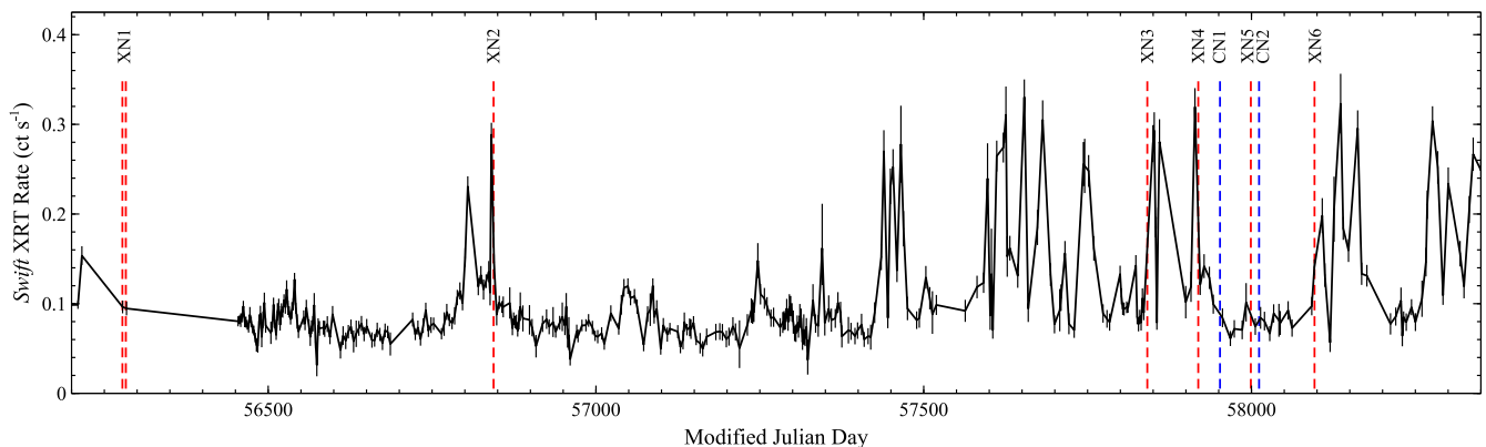
Figure 1. The long-term 0.3–10 keV X-ray lightcurve seen by Swift XRT since October 2012. The timing of the NuSTAR observations, which define the broad epochs considered here, are indicated by the red dashed lines for coordination with XMM-Newton , and blue dashed lines for coordination with Chandra . The period after MJD \sim 57400 shows enhanced variability, which is covered by a number of our broadband observations.
