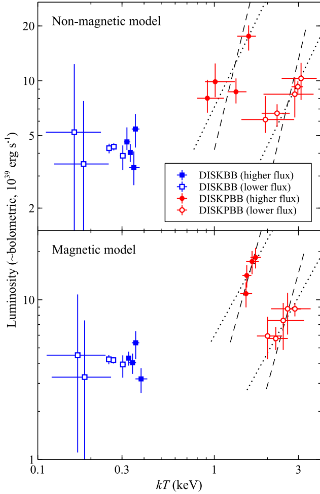
Figure 6. 0.001–100 keV ( i.e. \sim bolometric) luminosity vs temperature for both the DISKBB (blue squares) and DISKPBB (red circles) components from our multi-epoch spectral analysis with the models assuming the accretor is non-magnetic (top) and magnetic (bottom). No clear relation is seen for the DISKBB component (although this may be related to modelling issues, see Section 4). However, in both cases the results for the DISKPBB component appear to show distinct tracks at high and low luminosities (observed fluxes above and below F_{0.3-40.0}^{\text{obs}} = 5 \times 10^{-12} \text{ erg cm}^{-2} \text{ s}^{-1} ; full and open symbols, respectively), both of which are broadly consistent with L \propto T^4 (indicated with the dashed lines), and also with L \propto T^2 (dotted lines).
