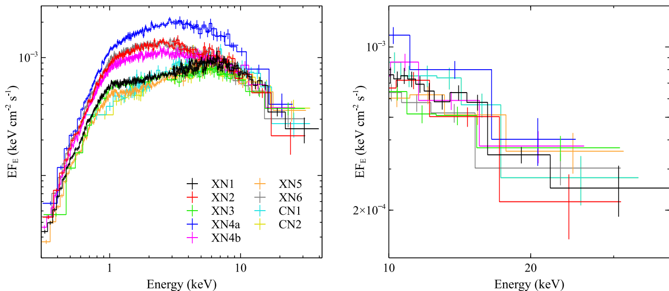
Figure 3. Left: The broadband spectral evolution displayed by NGC 1313 X-1. For clarity, we only show the EPIC-pn data for XMM-Newton and the MEG data for Chandra (where relevant), and the FPMA data for NuSTAR . Given the large number of datasets shown, we show the soft and hard X-ray coverage from each epoch in the same colour. The XMM-Newton data span the \sim 0.3 – 10.0 keV range, the Chandra data shown span the \sim 0.6 – 6.0 keV range, and the NuSTAR data span the \sim 3 – 35 keV range. Despite the strong variations at lower energies (below \sim 10 keV), the higher energy data (above \sim 10 keV) are relatively stable. Right: A zoom in on the high-energy ( >10 keV) data from NuSTAR (again, FPMA only for clarity), further demonstrating the relative lack of variability observed at these energies in comparison to the lower energy data. All the data have been unfolded through a simple model that is constant with energy, and have been further rebinned for visual purposes.
