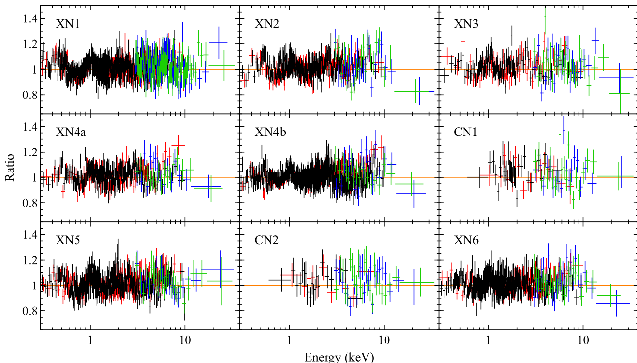
Figure 4. Data/model ratios for the nine broadband spectra extracted of NGC 1313 X-1 fit with the model assuming a non-magnetic accretor. Green and blue show data from the NuSTAR FPMA and FPMB detectors, respectively, while black and red show data from the EPIC-pn and EPIC-MOS detectors, respectively, for the XN epochs and from the MEG and HEG gratings, respectively, for the CN epochs. As with Figure 3, the data have been further rebinned for display purposes. The data/model ratios for the model assuming a magnetic accretor are extremely similar to those shown here.
