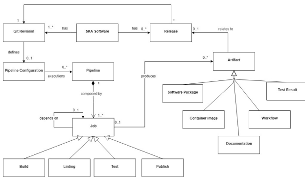
Figure 6: Data Model of the SKA CI-CD infrastructure.
