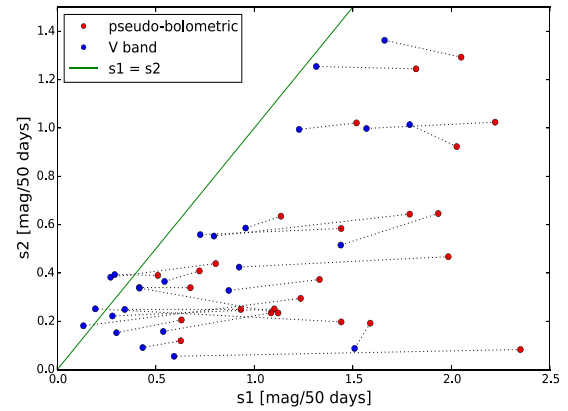
Figure 8. Parameters s_1 versus s_2 computed using the V band (blue) and the pseudobolometric light curve (red) for the sample of 22 SNe with multiband coverage. While s_2 remains nearly constant, s_1 increases if we use the integrated flux.
