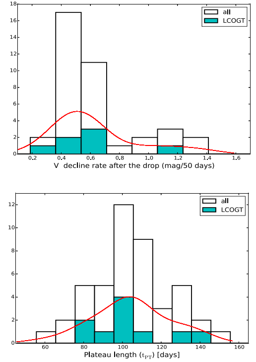
Figure D3. Top panel: distribution of light-curve decline rates s_{50V} after the drop for a sample of SNe II in V. Bottom panel: distribution of plateau length t_{PT} for a sample of SNe II in V. In red is the kernel density estimate using a Gaussian kernel for the same set of data.
