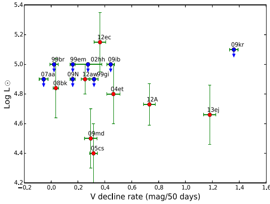
Figure 19. Progenitor luminosity from pre-explosion detection versus the V-band decline rate in 50 d. Progenitor data are from Smartt et al. (2009), Elias-Rosa et al. (2011), Fraser et al. (2011), Fraser et al. (2014), Maund et al. (2015), and Van Dyk et al. (2012).
