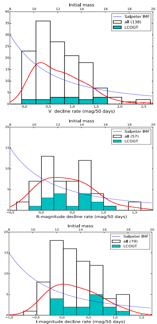
Figure D1. s 50 distributions for a sample of SNe II in V (top panel), R (central panel), and I (lower panel). In blue, we plot a Salpeter initial mass function to emphasize what the decline-rate distribution would look like if more-massive progenitors are related to faster decline rate SNe. In red is the kernel density estimate using a Gaussian kernel for the same set of data.
