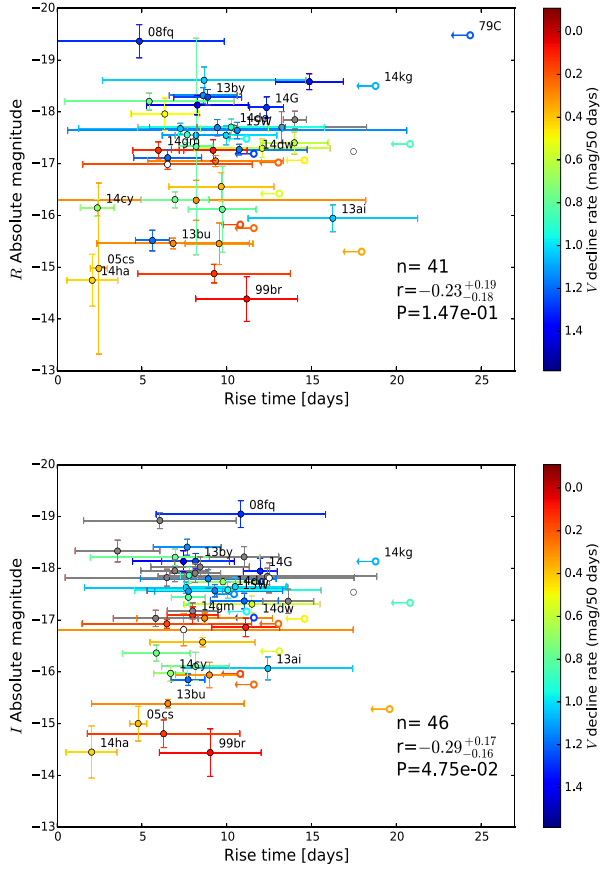
Figure D2. Absolute magnitude as a function of rise time for a sample of SNe II. Objects are colour-coded with the V-band decline rate s_{50V} . Top panel: R band. Bottom panel: I band. Data from Poznanski et al. (2015) have also been added in the I band.
