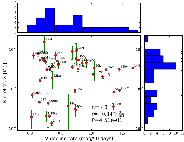
Figure 20. ^{56}\text{Ni} mass for a sample of SNe II versus the V-band decline rate in 50 d for a sample of SNe II. The data for the sample include SNe II from Hamuy (2003) and Spiro et al. (2014). For each panel, n is the number of events, r is Pearson's correlation coefficient, and P is the probability of detecting a correlation by chance.
