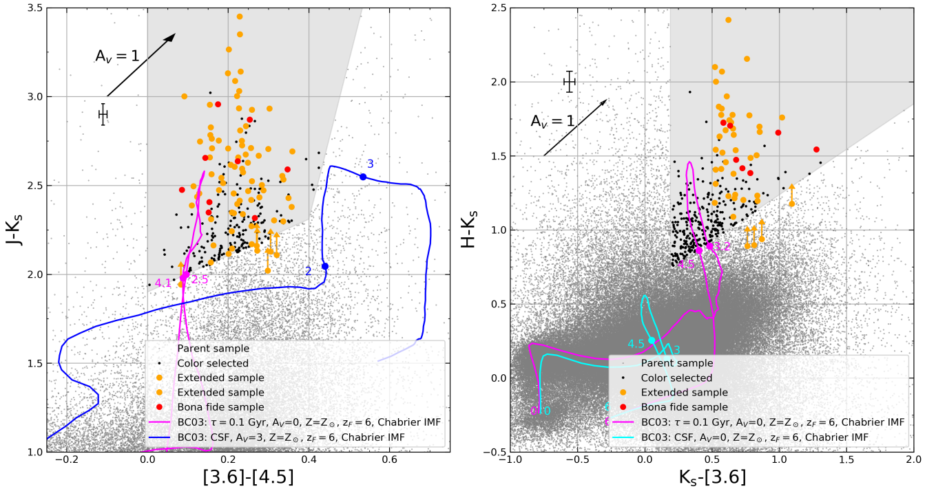
Fig. 3. Observed color-color diagrams. Left: JK_s[3.6]-[4.5] . Right: HK_s[3.6] . Gray shaded areas represent the color selection regions defined in Sect. 2 and the evolution of the colors of a quiescent and a star-forming galaxies are plotted as a reference. Gray points represent the whole parent sample selected as in Sect. 3.2, black points show the color-selected-only quiescent candidate. Red points are “bona fide” objects, while orange points belong to the “extended” sample, both defined in Sect. 4. The mean photometric errors of the color-selected candidates (black points) are also shown. Objects that are non-detected in one or more filters in the color-selected sample are not shown in order to improve clarity given their large number. Only undetected objects belonging to extended or bona fide samples are shown with arrows indicating the lower limits of the involved color. Non-detections correspond to <2\sigma .
