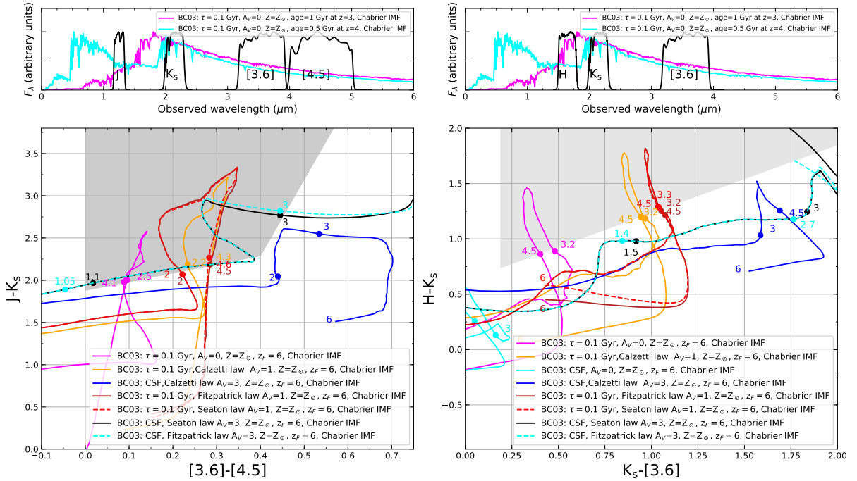
Fig. A.2. Effect of different extinction laws on JK_s[3.6][4.5] and HK_s[3.6] color-color diagrams. Top panels: two SEDs of quiescent galaxies (magenta and cyan lines), that is, a population 1 Gyr old redshifted to z = 3 and a population 0.5 Gyr old redshifted to z = 4 (i.e., z_{\text{form}} \approx 6 ) built with BC03 models. Bottom: evolution in the color-color plots for star-forming and passive galaxies. Tracks representing star-forming galaxies are shown in solid blue, solid black and dashed cyan lines, for the Calzetti, Seaton and Fitzpatrick laws, respectively, and their characteristics are shown in the inserted legends. Tracks for quiescent galaxies (with e -folding time of \tau = 0.1 Gyr and solar metallicity) are shown in solid magenta, solid orange, dashed red and brown for the Calzetti ( A_V = 0 and A_V = 1 ), Seaton and Fitzpatrick laws, respectively.
