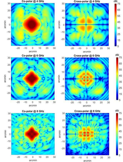
Fig. 14. Beam #1 patterns on the sky obtained by adding the far-field responses of 13 Vivaldi antenna elements feeding the SRT reflector from primary focus. Equal-weight was used to add the 13 far-fields. Co-polar (left) and cross-polar (right) beams on the sky at 4 GHz (top), 6 GHz (center) and 8 GHz (bottom).
