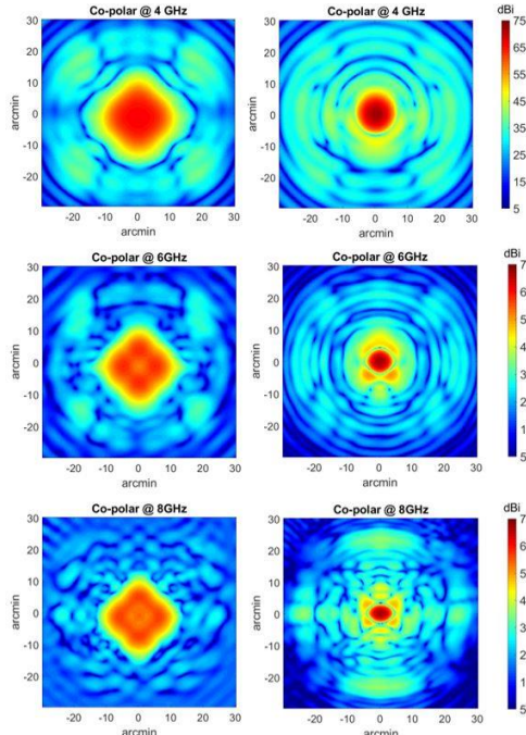
Fig. 16. Co-polar beam patterns of SRT by feeding 24 Vivaldi antennas with equal-weight (left panels) and with CFM weights (right panels) at 4 GHz (top), 6 GHz (center) and 8 GHz (bottom).
