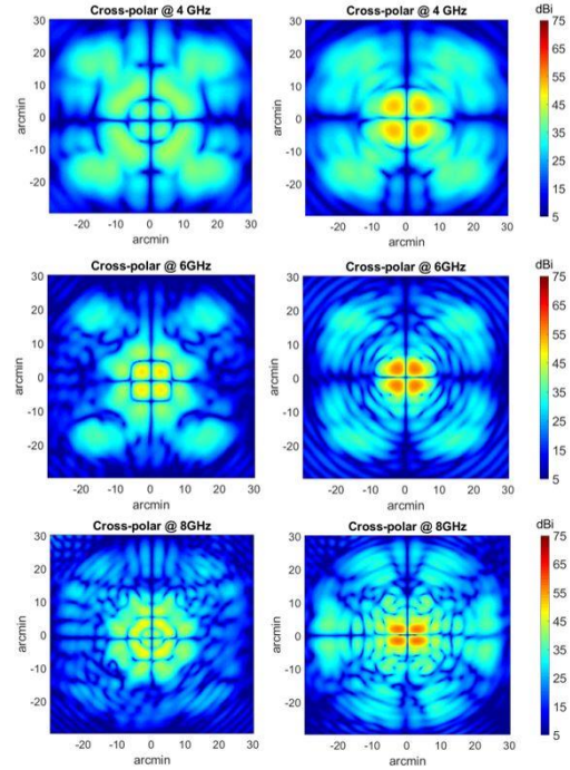
Fig. 17. Cross-polar beam patterns of SRT by feeding 24 Vivaldi antennas with equal-weight (left panels) and with CFM weights (right panels) at 4 GHz (top), 6 GHz (center) and 8 GHz (bottom).
