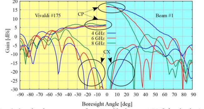
Fig. 9. Simulated antenna gains from Vivaldi element #175 (left side plots) versus Beam #1 (right side plots) formed by a linear combination of 13 elements equally fed. The plots refer to three following frequencies: 4 GHz (blue curve), 6 GHz (red curve) and 8 GHz (green curve).
