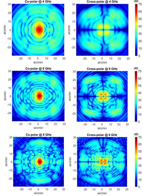
Fig. 13. Vivaldi element # 175 at SRT primary focus: co-polar (left) and cross-polar (right) beams on the sky at 4 GHz (top), 6 GHz (center) and 8 GHz (bottom).
