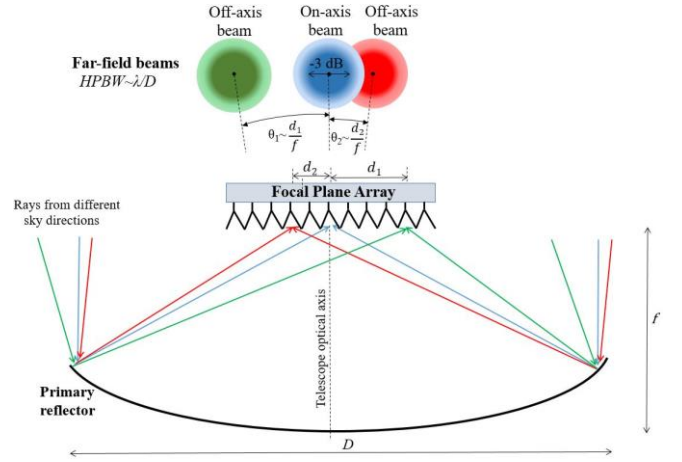
Fig. 1. Bottom: Schematic of a FPA at the primary focus of an axially symmetric single dish parabolic reflector with diameter D and focal length f . Plane waves from three different sky directions (on-axis in blue, off-axis in green and red) excite different areas of the FPA. Top: Far field patterns (angular size \approx \lambda/D ) and angular displacements from boresight ( \approx d/f ) resulting from the excitation of the different areas of the FPA at distance d from the axis.
