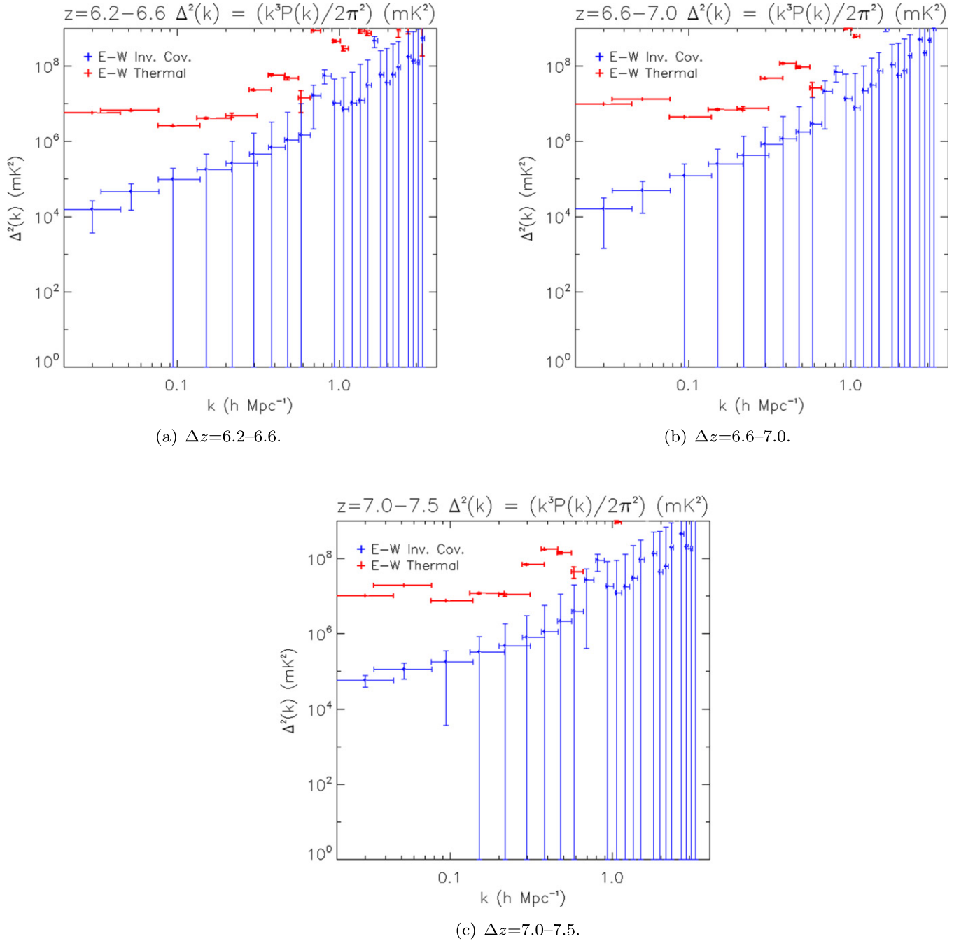
Figure 8. 1D spherically-averaged E-W polarization power spectra for three redshift ranges, corresponding to the upper, middle, and lower 10.24 MHz bands of the data. Both a thermal-noise-only (red) and a full foreground (blue) data covariance model has been used, as well as the full parameter space (no wedge excision).
