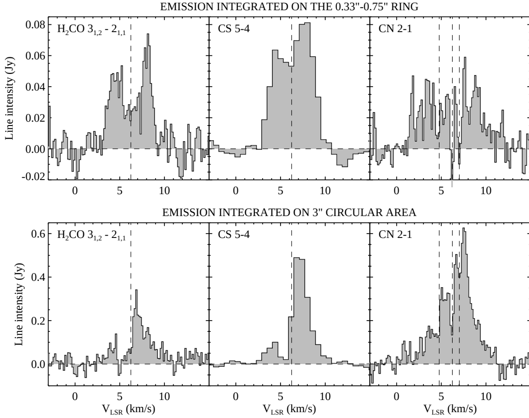
Fig. 3. \text{H}_2\text{CO } 3_{1,2}-2_{1,1} , CS 5-4, and CN 2-1 spectra integrated over a 0'.33-0'.75 ring area ( top panels ) and over a 3'' circular area ( bottom panels ). The vertical dashed lines indicate the systemic velocity, V_{\text{sys}} = +6.24 \text{ km s}^{-1} . For CN 2-1, the velocity scale corresponds to the brightest of the three hyperfine components at 226.87 GHz reported in Table 1 ( N=2-1 , J=5/2-3/2 , F=7/2-3/2 ), and the position of the two fainter components is indicated by the vertical dashed lines.
