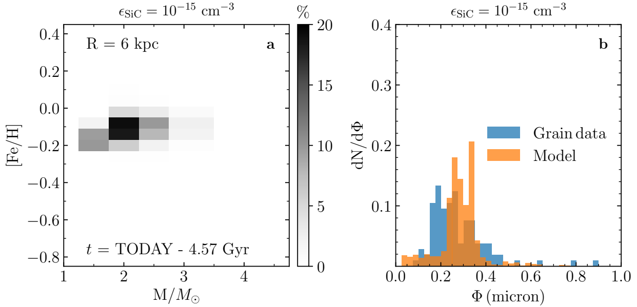
Fig. 3. Panel a: same as Fig. 2, but the percentages are weighted by the SiC grain yields of the corresponding AGB models (initial seed dust number \epsilon_{\text{SiC}} = 10^{-15} \text{ cm}^{-3} ). Panel b: corresponding distribution of SiC production vs. grain size (in diameter), compared to SiC grains identified in situ in primitive meteorites (see text for details).
