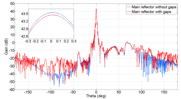
Fig. 2. Far field patterns at 1 GHz (Band 2) for the SKA dish with and without main reflector panel gaps.
