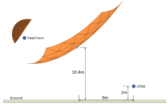
Fig. 1. Simulation setup including main and sub-reflector and feed horn at secondary focus. The LPDA antenna is introduced to illustrate the measurement setup as described in Section III (ground included for illustrative purposes).
