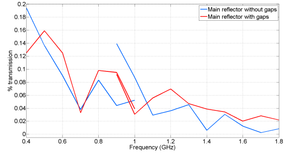
Fig. 4. Percentage transmission for SKA Band 1 and 2 of the main reflector with gaps compared to a solid reflector without gaps.
