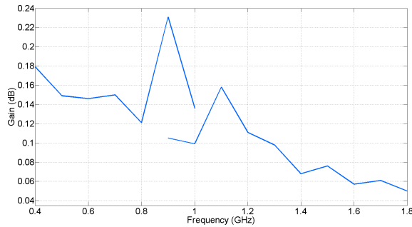
Fig. 3. Gain loss over frequency due to gaps in the main reflector.
