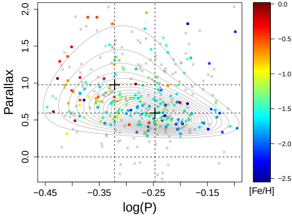
Fig. 4. Projection of a two-component 3D GM PDF fitted to the true values of ([Fe/H], \log P, \ln w) in data set B onto the plane period-parallax. The grey contours represent iso-probability lines. The coloured and grey points represent true and measured parallaxes, respectively. The black crosses indicate the median of the mean posterior distribution of each GM component. The colour encodes the metallicity.
