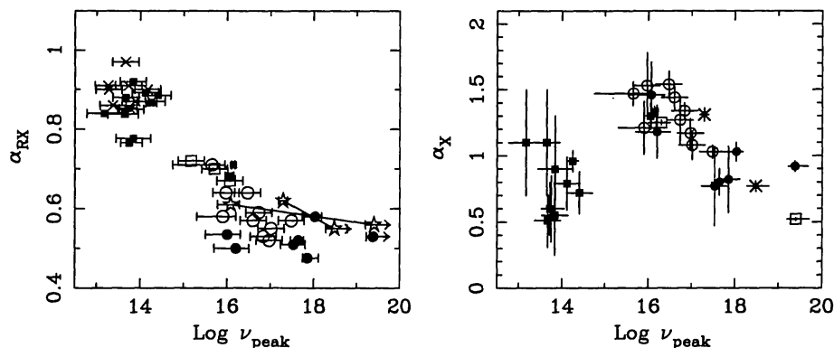
Figure 1. \alpha_{RX} and \alpha_x vs. \nu_{peak} for our 7 sources (filled circles) together with the HBL and LBL in Wolter et al. 1998 (open marks and crosses) and the 1 Jy BL Lacs data (Padovani et al. 2000, in preparation, filled squares). The “quiescent” and “flaring” states of Mkn 501 and 1ES 2344+514 are represented, on the left as stars with connecting lines, and on the right as open squares and asterisks, respectively.
