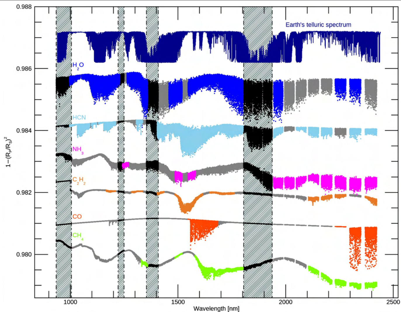
Extended Data Fig. 5 | Selection of the GIANO-B spectral orders. The Earth's telluric spectrum and the theoretical transmission spectra of H_2O , HCN, NH_3 , C_2H_2 , CO and CH_4 are shown from top to bottom in relative flux units. The colours display for each molecule the orders selected for the cross-correlation
