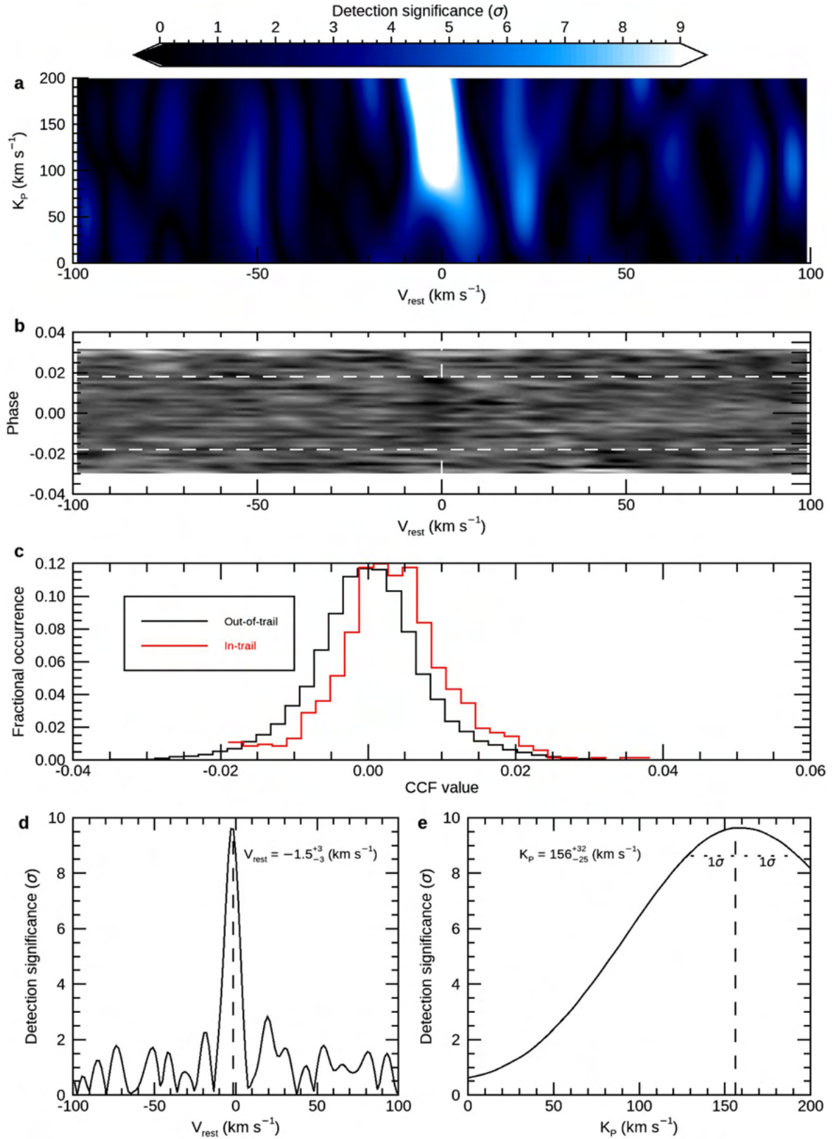
Extended Data Fig. 1 | Detection and analysis of the \text{H}_2\text{O} signal in the atmosphere of HD 209458b. a , Map of the significance of the cross-correlation values as a function of the planetary radial-velocity semi-amplitude K_p and the planet rest-frame velocity V_{\text{rest}} . b , Values of the cross-correlation function in the planet rest-frame as a function of the orbital phase and V_{\text{rest}} . The horizontal dashed lines denote the transit ingress and
