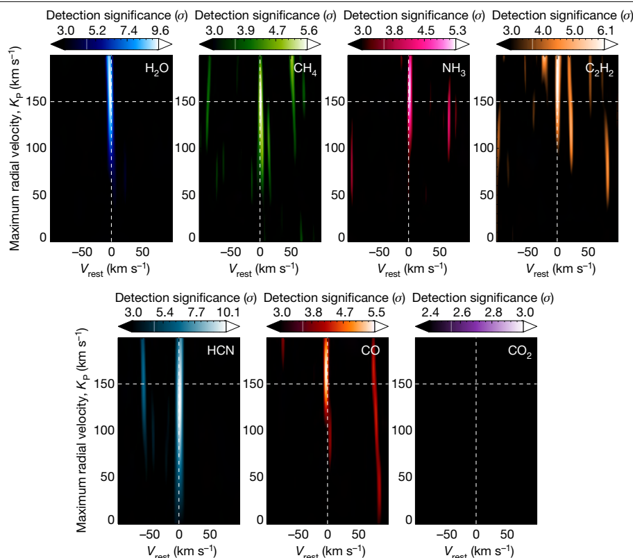
Fig. 1 | Detection significance for \text{H}_2\text{O} , \text{CH}_4 , \text{NH}_3 , \text{C}_2\text{H}_2 , \text{HCN} , \text{CO} and \text{CO}_2 . Each panel shows the significance of the cross-correlation of the GIANO-B spectra with isothermal atmospheric models, as a function of the planet's maximum radial velocity ( K_p ) and the planet's rest-frame velocity ( V_{\text{rest}} ). White
