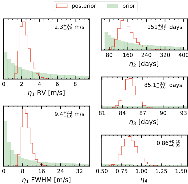
Fig. 6. Prior and posterior distributions for the hyperparameters of the GP in the two-planet model. Posterior estimates (median and 68% credible intervals) are shown in each panel. It should be noted that for \eta_3 and \eta_4 the full support of the prior is larger than what is shown.
