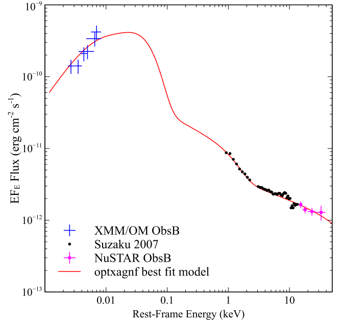
Figure 3. Optical to hard X-ray SED of PDS 456 obtained by combining the OM and NuSTAR data (blue and magenta respectively) from the XMM-Newton / NuSTAR observation in 2013 (ObsB) and the 2007 time-averaged spectrum from the Suzaku campaign (black). For clarity, the NuSTAR data is only plotted above 10 keV. The SED was fitted with the optxagnf model (red solid line). Note that the model is corrected for absorption (either Galactic or local to the source), the OM data has been dereddened as is described in Section 3.1 while the X-ray data have been corrected for a Galactic absorption column of 2.0 \times 10^{21} \text{ cm}^{-2} .
