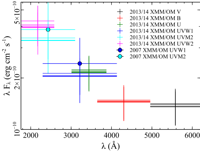
Figure 2. The XMM-Newton OM photometric data of PDS 456 taken between 2007 and 2014. Overall only small changes are observed in the optical/UV band, typically of the order of 5–20 per cent and are consistent within the uncertainties. Thus, when constructing the optical to hard X-ray SED, we can adopt the OM data from ObsB regardless of the fact that they are non-simultaneous with the 2007 Suzaku observation.
