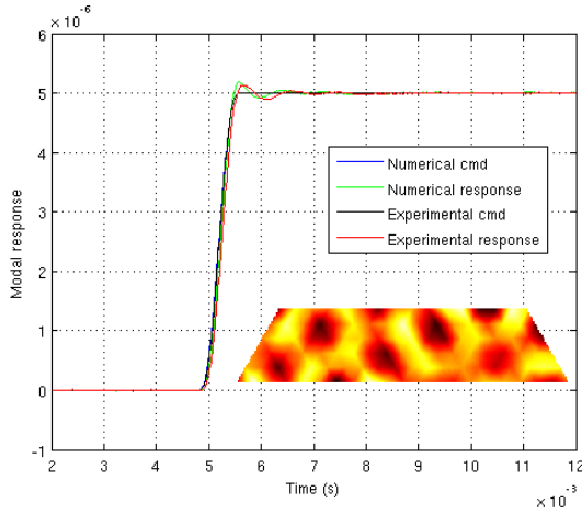
Figure 4. Mode 40 step response. Comparison between numerical and experimental results.
