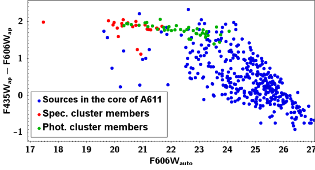
Figure 2. Colour–magnitude diagram for A611. We show all of the sources extracted in the core of A611 (blue), the cluster members with measured spectroscopic redshift (red) and the photometric candidate cluster members (green) included in the SL model.
