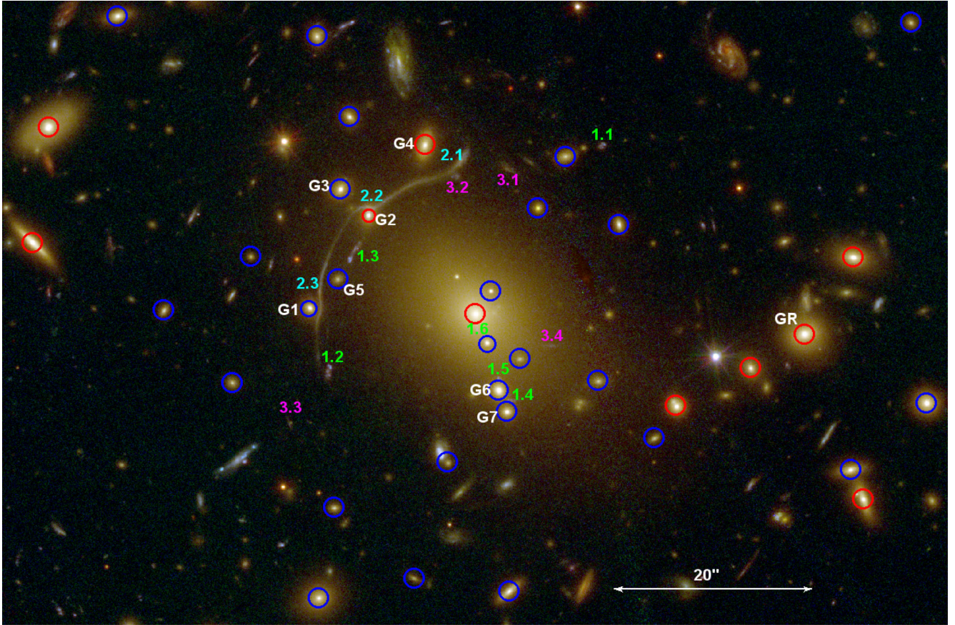
Figure 1. Colour composite image of the core ( \sim 1.5 \text{ arcmin} \times 1.5 \text{ arcmin} ) of A611 created using the CLASH HST data set: blue = F435W + F475W; green = F606W + F775W + F814W + F850LP; red = F105W + F110W + F140W + F160W. Blue circles mark the cluster members included in the SL analysis. Red circles mark the galaxies with measured central velocity dispersions. ‘GR’ indicates the galaxy used as reference for the luminosity scaling relation. ‘G1’ to ‘G7’ are the galaxies we model individually. The three multiply-lensed systems used in the SL analysis are labelled in green (system 1), cyan (system 2) and magenta (system 3). North is up and east is left.
