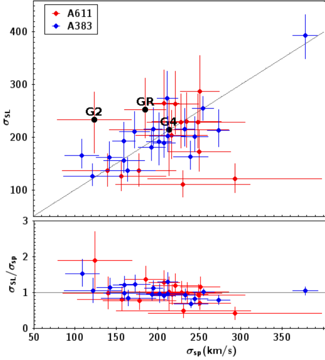
Figure 4. Spectroscopic velocity dispersions ( \sigma_{sp} ) versus the prediction from lensing. We show the relation for A611 (red) along with the individually optimized objects (black). For comparison we also show the results for A383 (in blue) from Monna et al. (2015). Note the tighter relation for A383.
