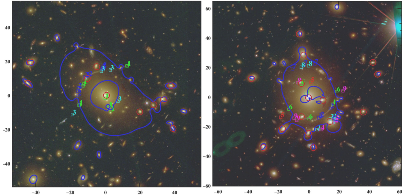
Figure 5. HST colour composite images of A611 ( z = 0.288 ; left) and A383 ( z = 0.189 ; right). We show the multiple image (numbered), the cluster members with measured \sigma_{sp} (red circles), and the critical lines for a source at redshift z_s = 2 (blue). Axis labels are in arcseconds with respect to the BCG.
