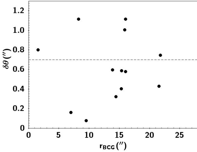
Figure 3. Distance \delta\theta between the predicted and observed multiple images as a function of the distance of the respective multiple images from the BCG. The multiple images are reproduced with mean accuracy of 0.7 arcsec.
