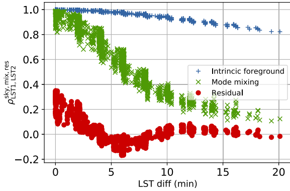
Figure 10. Correlation coefficient \rho_{LST1,LST2}^{sky,mix,res} as a function of LST difference for all the night, LST-binned data. Each marker symbol ('+', 'x' or 'o') represents an LST difference.
