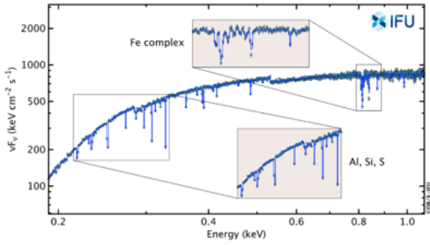
Fig. 2 A simulated Athena/X-IFU spectrum of a medium bright (fluence: 4 \times 10^{-7} \text{ erg cm}^{-2} ) z = 7 GRB afterglow characterized by deep resonant lines from the ISM of the GRB host galaxy. An effective intrinsic column density of 2 \times 10^{22} \text{ cm}^{-2} was assumed [credit: Athena/X-IFU Consortium].
