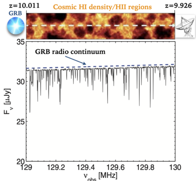
Fig. 4 Representation of the 21 cm absorption lines (known as the “21 cm forest”) produced by non-linear structures during the early stage of reionization [17].
