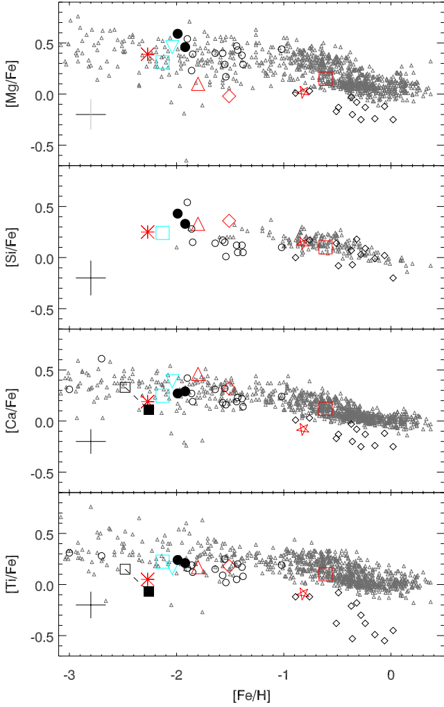
Fig. 4. [Mg/Fe] , [Si/Fe] , [Ca/Fe] , and [Ti/Fe] ratios plotted against [Fe/H] for the studied stars in NGC 5053 (filled black squares) and NGC 5634 (filled black circles), compared with Sgr dSph main body populations (open black circles, Sbordone et al., in prep.; open black diamonds, Sbordone et al. 2007), and mean values for five globular clusters related to Sgr dSph: Ter 8 (red asterisk), Arp 2 (open red triangle), M 54 (open red diamond), Pal 12 (open star), and Ter 7 (open red square). Small open gray triangles are Milky Way stars (Venn et al. 2004; Reddy et al. 2006). Large open cyan symbols are MW globular clusters NGC 6397 (square) and NGC 5897 (triangle). The large open black square connected by a dashed line with the filled black square represents the result for NGC 5053 when plotting [\alpha/Fe I] vs. [Fe I/H] , with the latter represented by the open symbol.
