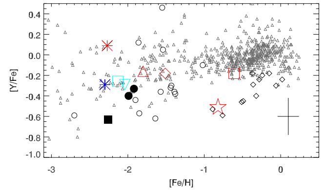
Fig. 6. [Y/Fe] plotted against [Fe/H] . Symbols are the same as in Fig. 4 except for the large blue asterisk, which represents the average Y abundance in Ter 8 as measured by Mottini et al. (2008). Here, in Fig. 7, and in Fig. 8 only the filled point appears for NGC 5053 since both Ba and Y are always compared to Fe II.
