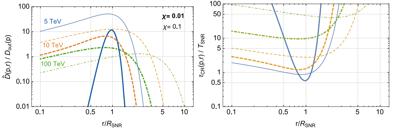
Figure C1. Left: spatial dependence of self-generated diffusion coefficient \hat{D}(p, r) divided by D_{\text{out}}(p) for \chi = 0.1 (thin lines) and \chi = 0.01 (thick lines), calculated by setting an acceleration spectrum with slope \alpha = 4 for the benchmark parameter values reported in Table 1. The parametrization of escape time adopted here follows equation (9), with \delta = 3 . The three sets of lines correspond to three different particle energies: 5 (solid), 10 (dashed), and 100 TeV (dot-dashed). Right: corresponding excitation time for the streaming instability in unit of SNR age ( 10^4 yr) and for the same energy values as the left-hand panel.
