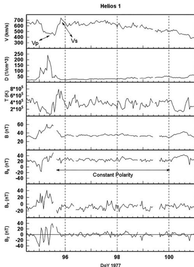
Figure 1. Helios 1 data for April 1977. HSSs are identified, from day 95 up to day 101.
