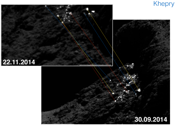
Fig. 5. Comparisons of OSIRIS NAC images of the cluster of bright spots 6 observed two months apart, which shows the stability of the bright features with time.
