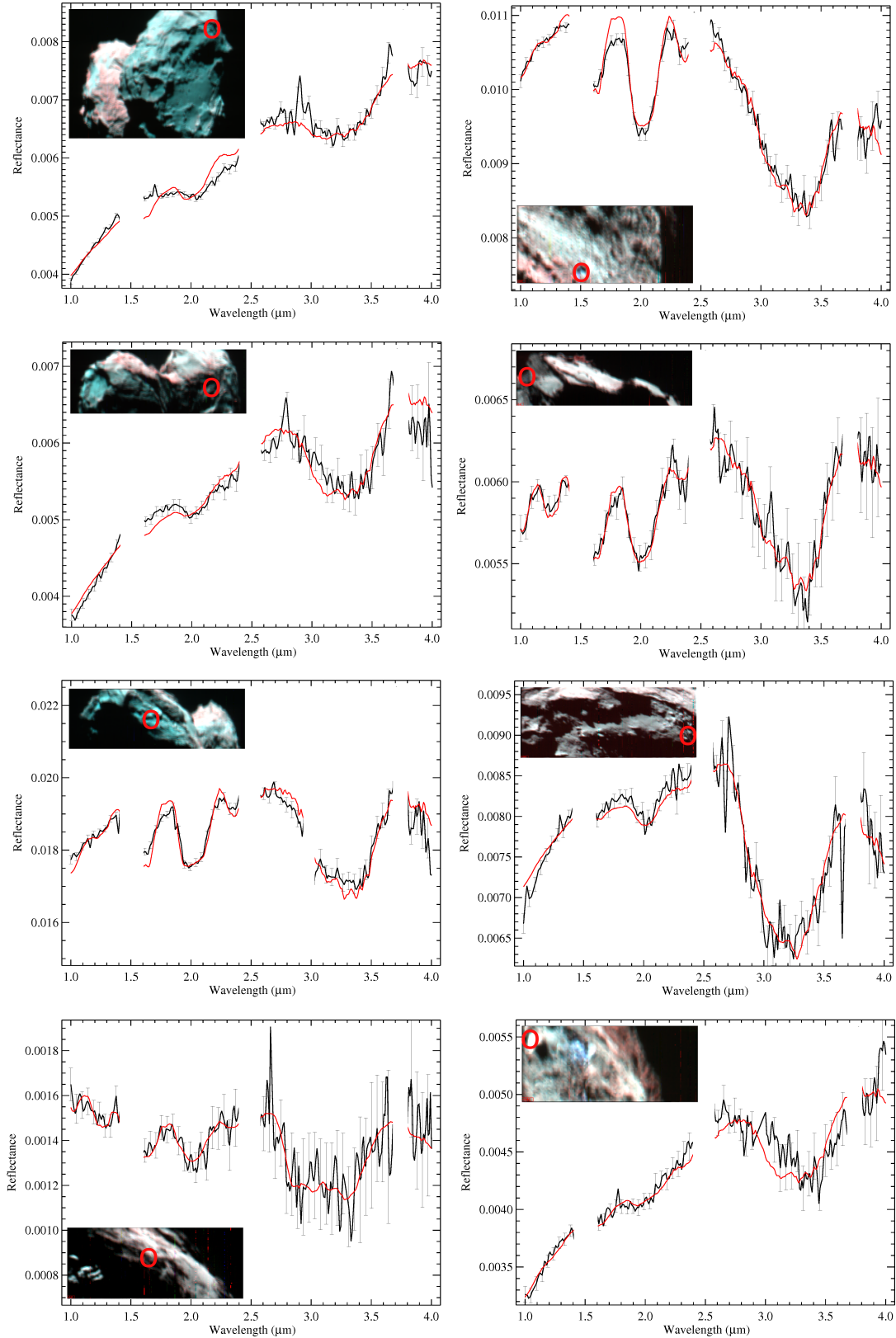
Fig. 4. VIRTIS-M infrared data of the eight spots. Spots 1-4 are shown on the left column from top to bottom. Spots 5-8 on the right column from top to bottom. Infrared images in the insert of the plot are built from a combination of spectral bands taken at 1.32\ \mu\text{m} (B channel), 2.0\ \mu\text{m} (G), 4.0\ \mu\text{m} (R). For each spot are reported the VIRTIS-M observed reflectance (black curve), not corrected for phase angle, and best fit (red curve) as derived on the pixels reported in Table 3 and indicated by the red circles on the images. The gaps in the spectral ranges correspond to order sorting filters junctions wavelengths that can produce unreliable features and for this reason are not taken into account in the analysis.
