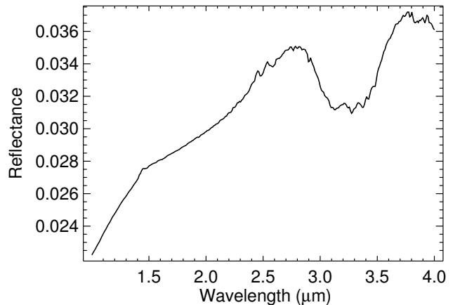
Fig. 3. Spectrum of “Dark Terrain” unit corresponding to the average spectrum of the comet’s surface.
