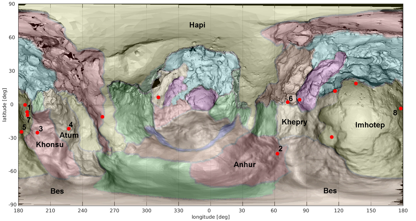
Fig. 1. Map of comet 67P/Churyumov-Gerasimenko resulting from merging a more detailed shape model SHAP4S (Preusker et al. 2015) for the northern hemisphere and shape model SHAP5 (Jorda et al. 2016) for the southern hemisphere. In red are reported the selected bright spots, based on OSIRIS images and a spectro-photometric analysis, considered as good targets to be investigated by an analysis of VIRTIS data, plus the two bright spots analysed by Filacchione et al. (2016a). The numbers (1-8) represent the spots with positive detection of H 2 O ice by VIRTIS analysis discussed in this paper.
