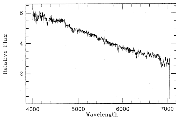
Fig. 5. Spectrum of Nova Muscae 1991 in the range 4000–7000Å obtained on May 19 at the ESO 3.6m telescope under non-photometric conditions.
