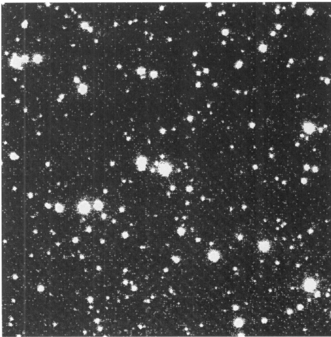
Fig. 1a. Nova Muscae 1991 during its flare up in early January 1991 in the southern constellation of Musca. The CCD frame was secured on 15.3 January 1991, (seeing 0.9 arcsec); with the ESO New Technology Telescope (5 sec exposure in R). The nova is the bright object at the centre. Fig. 1b. Reproduction of an earlier red-sensitive ESO Schmidt plate (120 min exposure on IIIa-F + RG630; 29 January 1976). The pre-nova is faintly visible.
