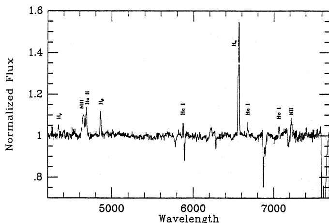
Fig. 4. Continuum normalized spectrum of Nova Muscae 1991 obtained on January 15.3 UT at NTT.
