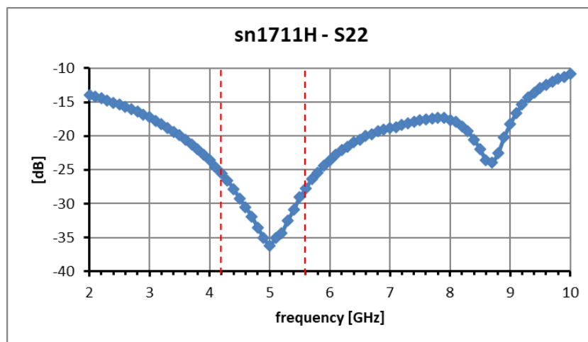
Fig. 4.3 sn1711H caldo, S22, V_d=1.35V I_d=45mA
