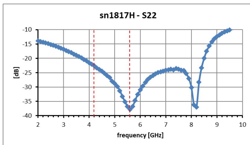
Fig. 4.13 sn1817H caldo, S22, V_d=1.35V I_d=45mA
