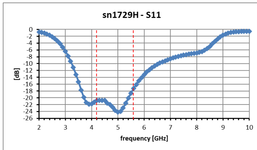
Fig. 4.6 sn1729H caldo, S11, V_d=1.35V I_d=45mA
