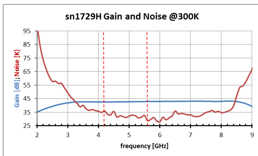
Fig. 4.10 sn1729H caldo, Gain&Noise, V_d=1.35V I_d=45mA
