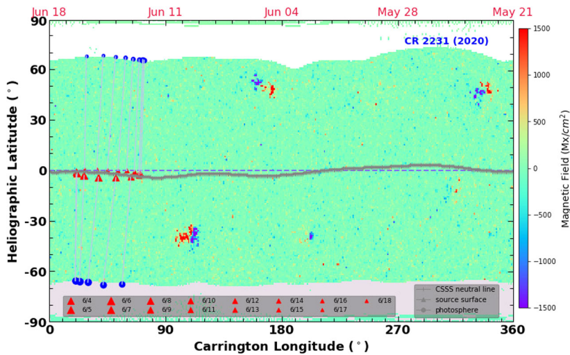
Figure 20 The locations of Parker Solar Probe (4–18 June 2020), mapped back to the Sun using the Current Sheet Source Surface model (CSSS, developed by Zhao and Hoeksema, 1995, see also Poduval and Zhao, 2014, Poduval, 2016, Chandorkar et al., 2020), superimposed on an SDO/HMI synoptic magnetogram (Carrington rotation 2231, downsampled to one-degree resolution). The red triangles are the map-back locations at 15 R_{\odot} (the CSSS source surface) assuming a constant radial solar-wind speed of 395 \text{ km s}^{-1} . These are joined to their photospheric foot points (blue filled circles) by thin gray lines to indicate connectivity. The CSSS deduced open magnetic-field regions (coronal holes) are shown in white and gray in northern and southern hemispheres, respectively, with the magnetic polarity inversion line (heliospheric current sheet) marked with dark-gray plus symbols. Figure courtesy of B. Poduval.
