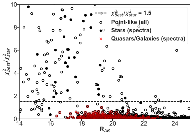
Figure 14. Ratio of \chi^2 values for best-fit quasar/galaxy model ( \chi^2_{\text{best}} ) to best-fit star ( \chi^2_{\text{star}} ) against R_{\text{AB}} magnitude. Low ratios indicate secure quasar/galaxy identifications; red crosses show spectroscopically confirmed quasar/AGNs. Black filled points show spectroscopically confirmed stars, only five of which (all cataclysmic variables) have ratios < 1.5 and thus are misclassified (10% of the 57 stars with spectra).
