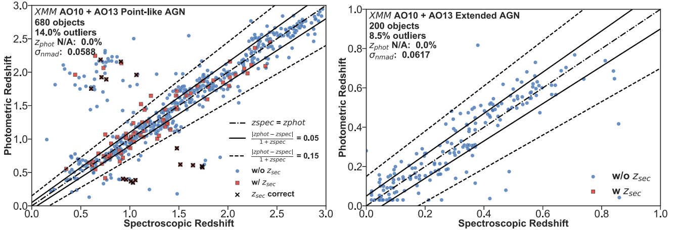
Figure 11. Spectroscopic vs. photometric redshift for point-like (left) and extended (right) sources in the uniform XMM-Newton fields. The results in the other fields are very similar, as can be seen in Table 7. Black crosses indicate cases where the primary redshift is incorrect and the secondary redshift is correct (i.e., it lies within the dashed black lines). The quantity “ z_{\text{phot}} \text{ N/A} ” reports the percentage of sources for which we are unable to calculate photometric redshifts altogether due to data in very few bands or not having an appropriate SED template in our template library.
