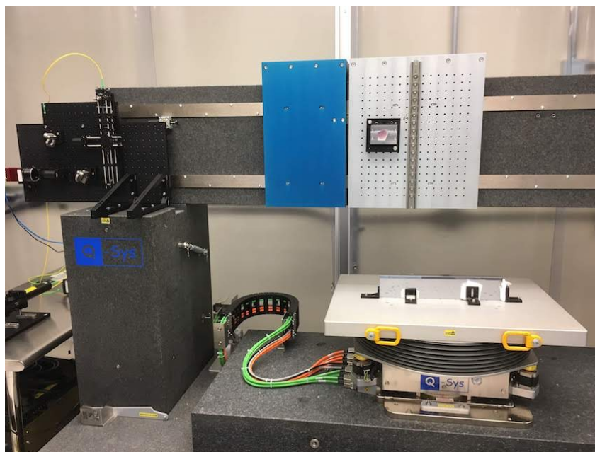
Figure 1. The new LTP in the LCLS labs. The fixed optical head (see detail in Fig. 4) is visible on the left side. The gantry system performs the scan of the pentaprism (on the central stage) over the mirror length. The mirror under test can be moved in the other five degrees of freedom by another granite stage and the tip-tilt-rotate table which the sample is mounted on.
