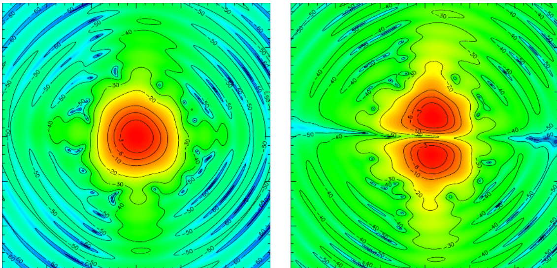
Figure 9 Main Beam 3 at 100 GHz – PG28. Co and Cross polar component.
