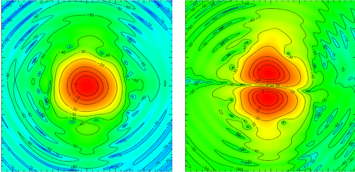
Figure 8 Main Beam 3 at 100 GHz – PG21. Co and Cross polar component.
