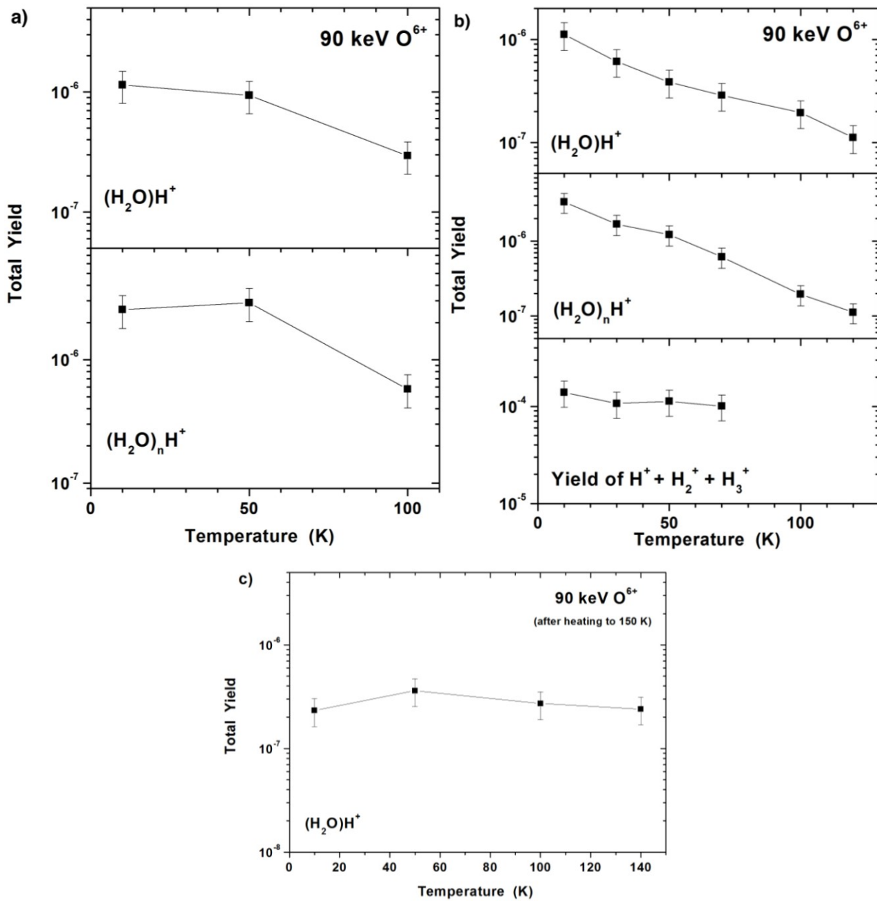
Figure 5. Secondary Total Ion Yields calculated for the most abundant secondary ion (H_3O)^+ , for the total amount of clusters (H_2O)_n H^+ ( n=1-8 ) and for the hydrogen ions ( H^+ , H_2^+ , H_3^+ ); emitted from: a) amorphous ice water, b) fresh ice and c) crystalline ice water.
