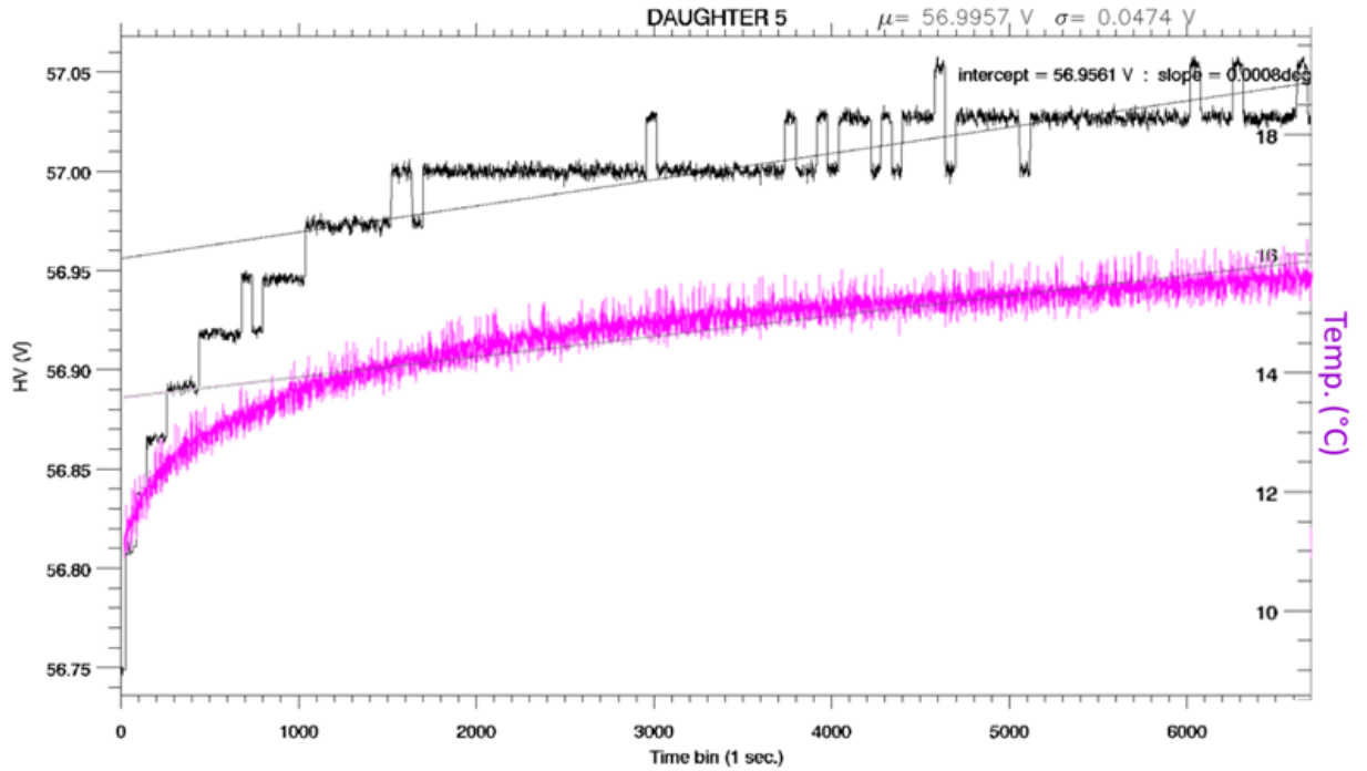
Figure 14: Temperature time profile of the central temperature sensor and resulting SiPM Vop adjustment. It should be noted that the V_{op} adjustment steps follow the trend of the temperature profile.
