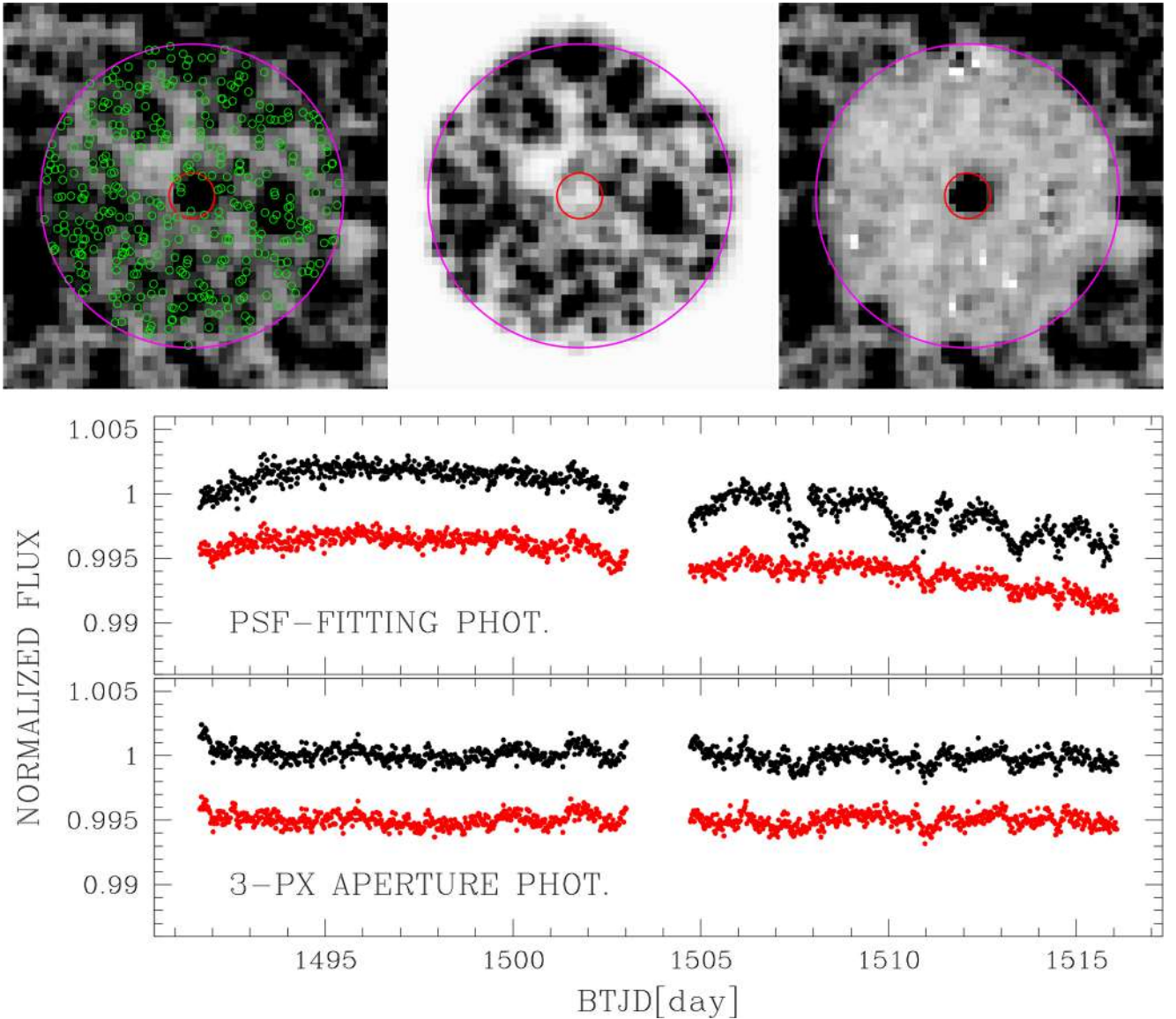
Figure 2. From FFI to the final light curve. Top panels: example of neighbour subtraction. The left-hand panel shows the original FFI (tess2019009222936-s0007-1-1-0131-s_ffic.fits) centred on the star Gaia DR2311138192822301184, a possible cluster member of Gulliver47; red circles show the photometric aperture used to analyse this star, and green circles show the neighbours located within a radius of 20 pixels (magenta circle) from the target star. The middle panel shows the models of the neighbours subtracted from the FFI; the right-hand panel shows the FFI after neighbour subtraction. Bottom panels: the PSF fitting and 3-pixel aperture photometry light curves of the star Gaia DR2311138192822301184 before (black points) and after (red points) the systematic correction.
