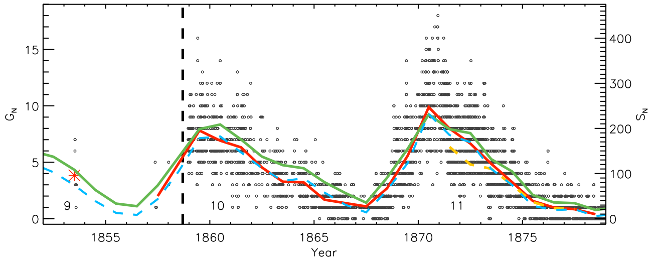
Figure 14. Group numbers derived from the drawings of the Secchi collection in this study (daily counts are shown in gray and annual mean values in red). Also shown are the annual values of the group number series by Chatzistergos et al. (2017, solid green) and S_N (the values are given in the right axis; dashed light blue) as well as the raw group counts of Secchi (dashed yellow) from the Vaquero et al. (2016) database. The vertical dashed black line separates the sporadic data prior to 1858 December and the regular ones afterward. The numbers at the lower part of the figure denote the conventional solar cycle numbering.
