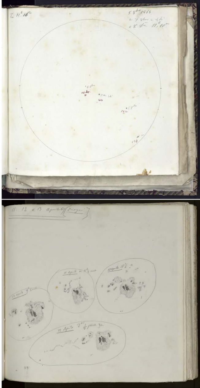
Figure 5. Examples of drawings reporting the evolution of sunspot groups from 1865 October 5–8 (top) and from 1869 April 11–13 (bottom).
