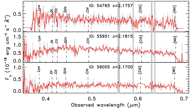
Fig. B.3. VIMOS spectra (gray line) of three member candidates with z = 2.164\text{--}2.19 in the 10' \times 12' region centered at \alpha = 150.465^\circ , and \delta = 2.31^\circ where G237 is located. The red lines are smoothed spectra. The vertical dashed lines represent the location of the main spectral lines as annotated. Source IDs and spectroscopic redshifts are annotated in each panel. Regions contaminated by bright sky lines are highlighted with vertical gray bars.
