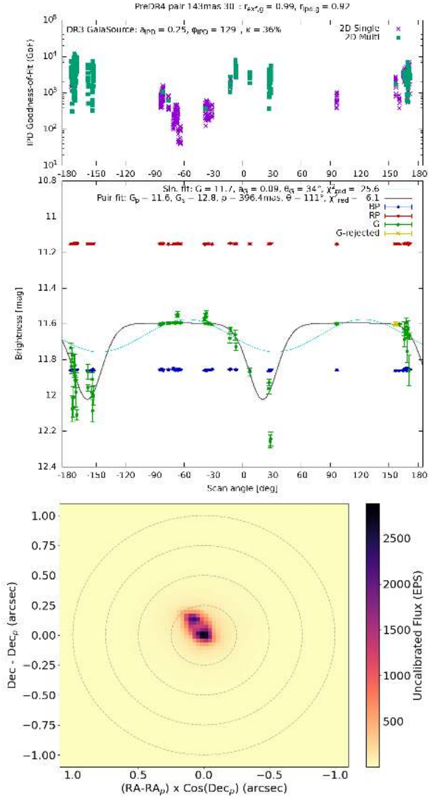
Fig. B.2. SourceID 378810450446502400: Scan-angle signatures and image reconstructed by SEAPipe.
