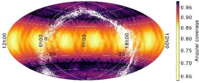
Fig. 5. Sky distribution in ecliptic coordinates of extragalactic sources analysed in terms of surface brightness profile in Gaia DR3, colour-coded with the angular coverage of the sources. The non-linear shader table reveals the NSL pattern.
