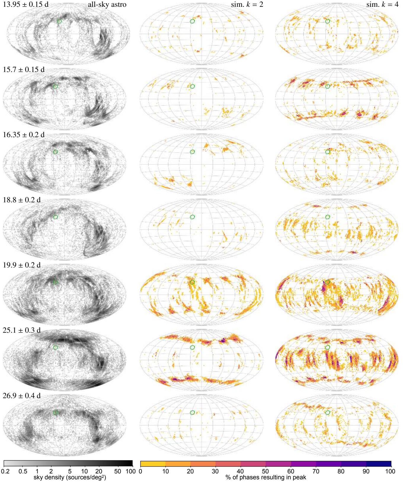
Fig. C.6. Ecliptic Aitoff projection of the astrometric period data presented in Fig. 24. Left: Source density of the astrometric peaks for the all-sky sample (top panel of Fig. 24). Right: Result of the all-sky uniform simulations of our noiseless sampled bias model (panels 2 and 3 of Fig. 24). They are colour-coded with the percentage of phases (position angles) that results in this peak: a low value means that only specific phasing of the scan-angle signal will result in a particular peak being observed at the given location. The green circle indicates the location of the GAPS catalogue. In all sky plots longitude zero is at the centre and increases to the left.
