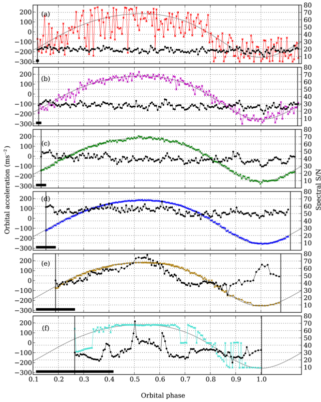
Figure A2. Detected orbital acceleration and S/N at various orbital phases for test data set 2. Each panel corresponds to progressively longer values of r_{\text{orb}} , from (a) 0.0095, (b) 0.019, (c) 0.038, (d) 0.076, (e) 0.15 to (f) 0.30.
