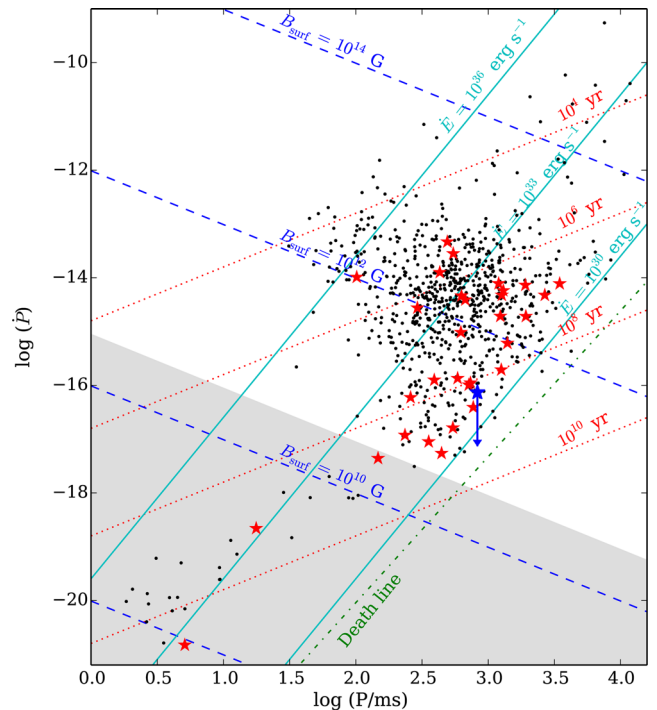
Figure 12. P – \dot{P} diagram showing the known pulsar population (black) within the HTRU Galactic plane survey region. The 32 new discoveries that have now preliminary timing solutions are denoted by red stars, except PSR J1829–1009 for which a 2\sigma upper limit is shown by a blue star. Lines of constant characteristic ages are shown as red dotted lines, and it can be seen that the newly discovered pulsars appear to be of an older population. In addition, lines of constant spin-down energies are shown as cyan solid lines and surface magnetic field strength as blue dashed lines. The death line as described in Chen & Ruderman (1993) is shown as green dot-dashed line. We define ‘recycled pulsars’ to be those with B_{\text{surf}} \leq 3 \times 10^{10} G as indicated by the shaded region.
