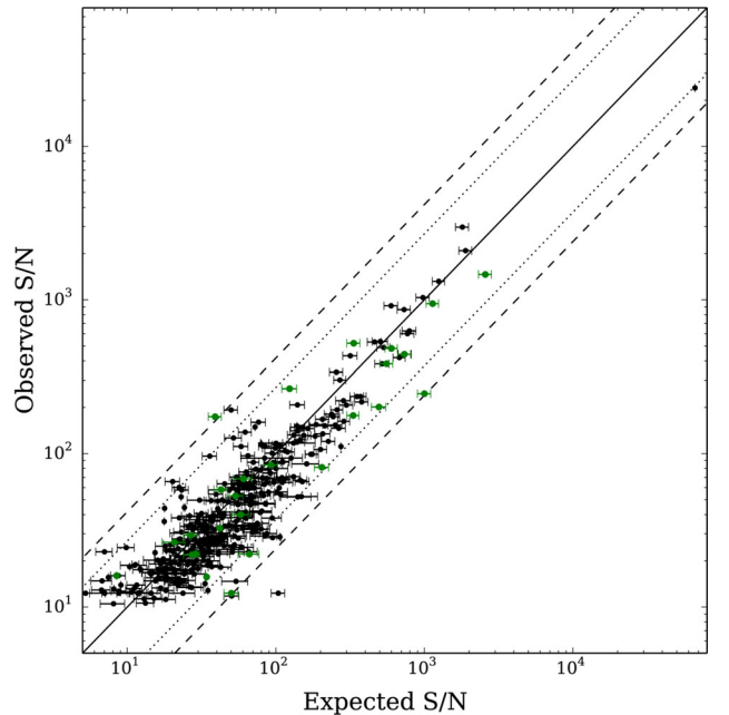
Figure 7. A comparison of the observed S/Ns of known pulsar redetections with their predicted values. The solid line shows the expected 1:1 correlation. The dotted and dashed lines mark the region containing 95 and 99 per cent of the data points. Pulsars with \text{DM} \leq 100 \text{ cm}^{-3} \text{ pc} are potentially affected by scintillation and are coloured in green. The error bars reflect the published uncertainties in the pulsar flux densities from PSRCAT.
