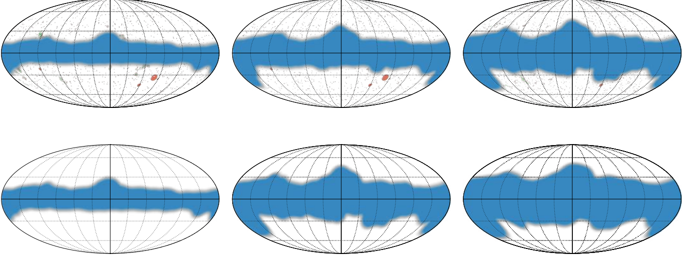
Fig. 29: Masks used in the Plik likelihood in temperature (top) and polarization (bottom). From left to right we show masks for 100 GHz (T66 top, P70 bottom), 143 GHz (T57 top, P50 bottom), and 217 GHz (T47 top, P41 bottom). Blue correspond to the Galactic (dust) mask, green is CO, and orange is the point-source and extended-source mask.
