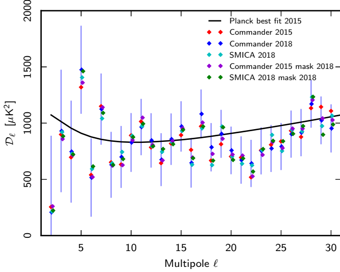
Fig. 2: TT angular power spectra ( D_\ell \equiv \ell(\ell+1)C_\ell/2\pi ) of the available low- \ell component-separated maps: Commander 2018 (blue points); Commander 2015 (red points); SMICA 2018 (cyan points); and Commander 2015 and SMICA 2018 masked with the 2018 Commander mask (purple and green points, respectively).
