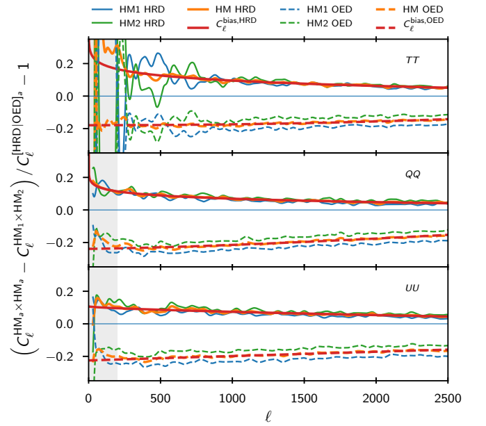
Fig. 48: Correction ( C_\ell^{\text{bias}} ) for the noise estimates based on HRDs (solid lines) and OEDs (dashed lines), as described in Eqs. (35) and (36). Blue and green lines show the two contribution to the bias estimates (i.e., for HM1 and HM2), showing that the bias is similar enough in each so that we can use the mean for the correction (orange line). The model fit (red) is obtained by restraining the fit to the non-shaded region ( \ell > 200 ). As we found in PPL15, HRD noise estimates are found to be biased low (due to correlations between half-ring maps, as explained in Planck Collaboration VI 2014). OED noise estimates, on the other hand, are biased high (in particular in polarization). Once the corresponding correction is applied to either case (HRD or OED), the overall noise models are similar. We only present here the 100-GHz channel results where the effect is the most striking. OEDs have very low anti-correlation for TT at 143 GHz and a slight correlation at 217 GHz, while the QQ and UU equivalents are still anticorrelated at all frequencies.
