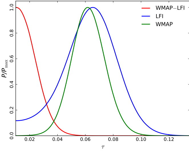
Fig. 28: Posterior distributions for \tau estimated from: the LFI baseline likelihood ( \tau = 0.063 \pm 0.020 ); the WMAP data set smoothed with a cosine window, cleaned as given in Table 12, and masked with the analysis mask P06 ( \tau = 0.062 \pm 0.012 ); and the difference between these two data sets, WMAP – LFI, to which we apply a mask given by the intersection of the R1.8x and P06 masks ( \tau \leq 0.033 at 95 % CL).
