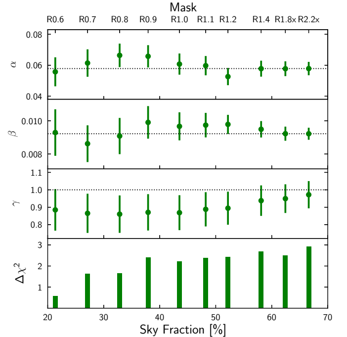
Fig. 22: Scaling coefficients for synchrotron ( \alpha ), dust ( \beta ), and the amplitude of the gain template ( \gamma ) estimated on several masks. Dotted lines mark the values of the coefficients for mask R2.2x, which are the ones we use to build the cleaned data set for the pixel-based likelihood. The bottom panel shows the \chi^2 excess of the fit, defined as \Delta\chi^2 = (\chi^2 - N_{\text{dof}}) / \sqrt{2N_{\text{dof}}} .
