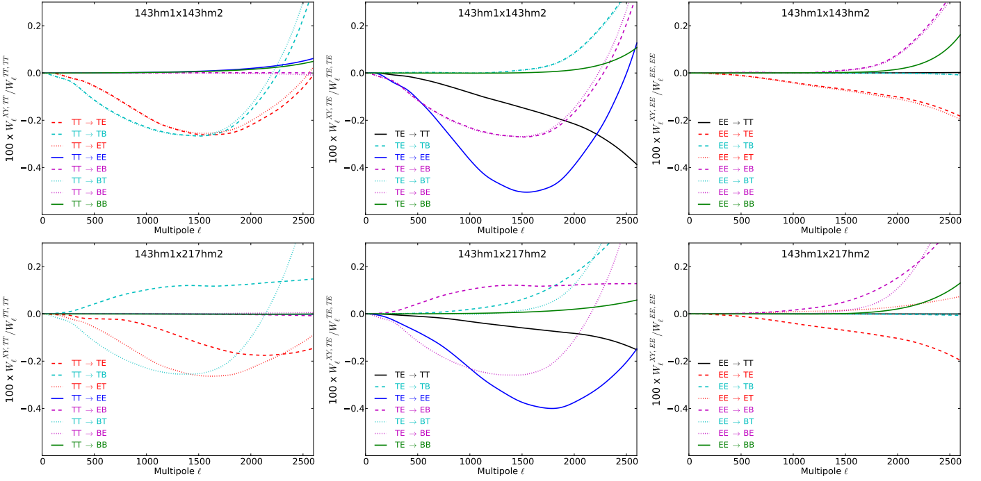
Fig. 50: Elements of the beam matrices \widehat{W}^{XY, TT} \equiv W^{XY, TT} / W^{TT, TT} (left panels), \widehat{W}^{XY, TE} (middle panels), and \widehat{W}^{XY, EE} (right panels), for the cross-analysis of 143-HM1 and 143-HM2 (upper panels) and of 143-HM1 and 217-HM2 (lower panels).
