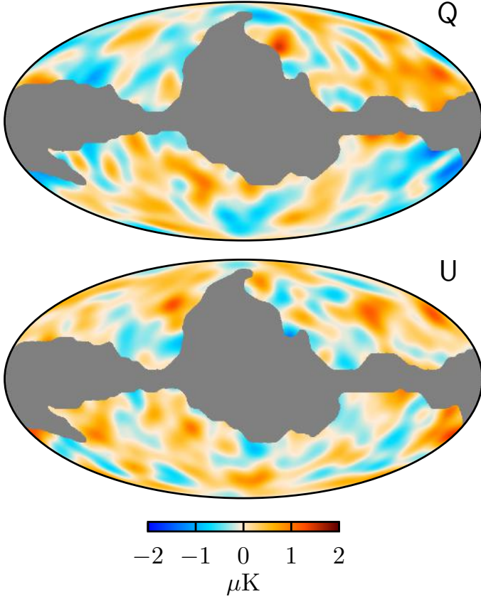
Fig. 23: Foreground-cleaned 70-GHz maps of the Stokes parameters Q (top) and U (bottom) on 62.4 % of the sky (mask R1.8x). In order to highlight the largest angular scales relevant for the low- \ell likelihood, these maps have been smoothed with a Gaussian filter of \text{FWHM} = 10^\circ . As a reference, for \tau \approx 0.06 the expected range for the signal is \pm 0.4 \mu\text{K} .
