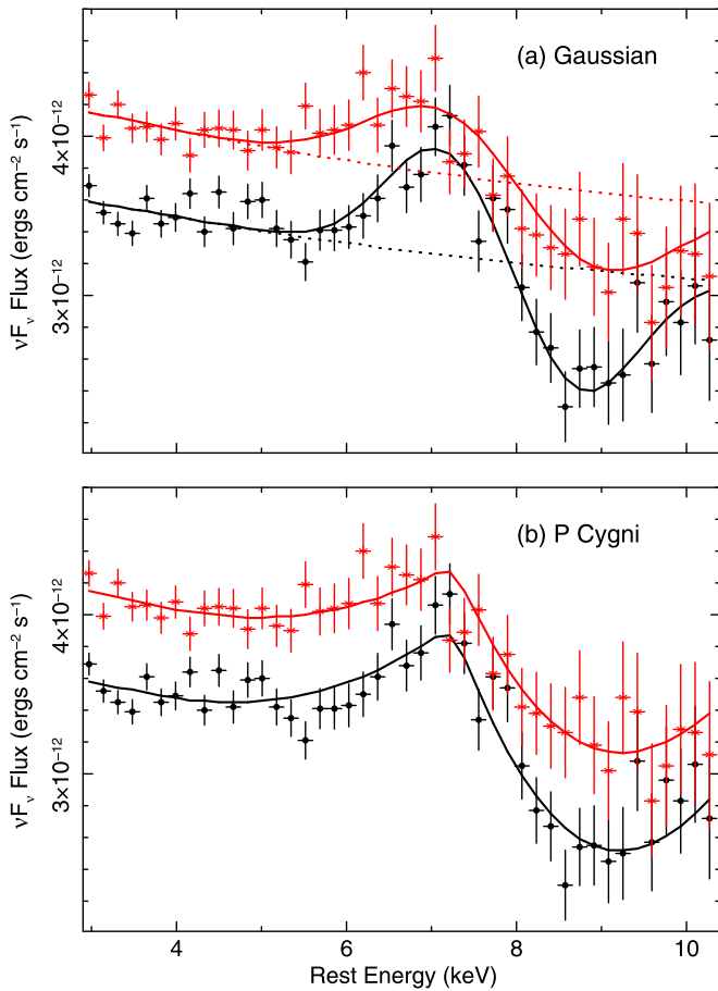
Figure 2. Fluxed spectra of IZw 1 fitted with two profiles, (a) a Gaussian profile in emission and absorption and (b) a P Cygni wind profile. OBS 1 spectra are in black and OBS 2 spectra in red. The Gaussian profile in panel (a) clearly shows the broadened emission vs. blueshifted absorption in the iron K band, while the best-fitting power-law continuum is shown as a dashed line. The best-fit centroid energy of the blueshifted absorption trough, near 8.6 keV, when compared to the expected energies of He- or H-like iron (6.70 or 6.97 keV), indicate the presence of a fast wind. The P Cygni profile in panel (b) is fitted with the model of Done et al. (2007) from a spherical wind reaching a terminal velocity of v_\infty \sim 0.35c . See Section 3 and Table 2 for details of the model parameters.
