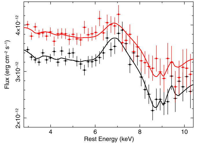
Figure 5. The 2015 pn spectra of I Zw 1, fitted with the XSTAR model described in Section 4.2 and with the parameters listed in Table 3. The emission and absorption model applied to the data has a velocity broadening of 25,000 \text{ km s}^{-1} , in order to account for the profile width. A fast absorber, of outflow velocity v/c = -0.265 \pm 0.010 , accounts for the broad absorption trough, while the iron K emission results from the subsequent reemission from the wind. Note the very weak emission feature at 9.3 keV is the radiative recombination emission from Fe XXVI.
