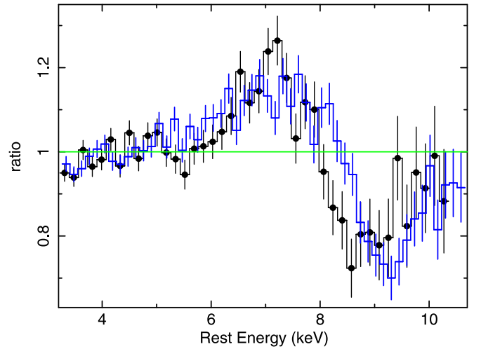
Figure 11. Comparison between the Fe K wind profiles in I Zw 1 and the quasar PDS 456. The black circles show the I Zw 1 2015 OBS 1 profile, while the blue points show the pn profile of PDS 456, from the third and fourth observations of the 2013–2014 XMM-Newton campaign (Nardini et al. 2015). Both AGNs are plotted in their respective rest frames ( z = 0.184 for PDS 456, z = 0.0611 for I Zw 1) and are shown as a ratio against a simple absorbed power-law continuum. The profiles show strong similarities; both require broadened emission centered near 7 keV as well as a broad, blueshifted absorption trough above 8 keV, of similar optical depth. The blueshift of the 2013 PDS 456 profile is slightly higher than in I Zw 1, suggesting a somewhat higher outflow velocity. The wind energetics are similar for both AGNs, with the mass outflow rate and kinetic power typically of 10% Eddington (see Section 6.1). Overall, I Zw 1 may represent a lower mass analog of the powerful disk wind in PDS 456.
