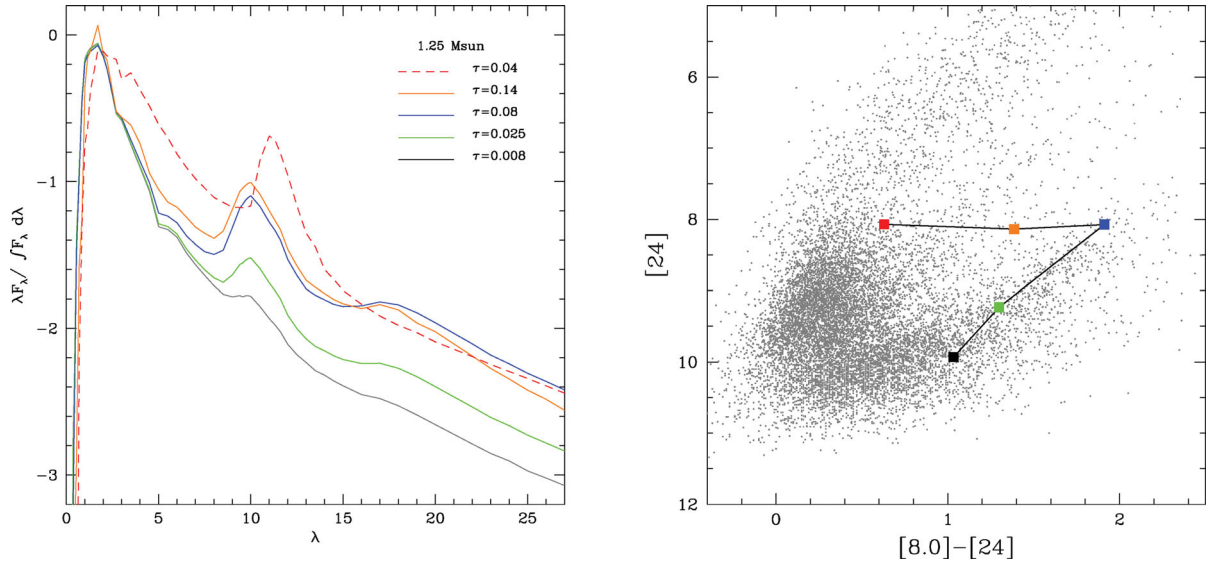
Figure 9. Left panel: the synthetic SED of a 1.25\text{-}M_{\odot} model of metallicity Z = 8 \times 10^{-3} at various evolutionary stages. The O-rich phase of the star is represented with a solid line, while the dashed line refers to the C-rich stage. Right panel: the theoretical track in the [8.0] - [24] versus [24] colour-magnitude diagram, where the coloured points refer to the corresponding spectra in the left panel.
