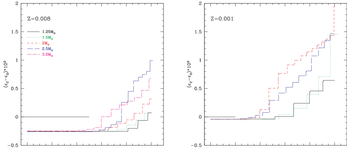
Figure 2. The evolution of the relative excess of carbon with respect to oxygen (see text for definition) during the AGB phase of stars with masses in the range 1.25\text{--}3\,M_{\odot} and metallicity Z = 8 \times 10^{-3} (left panel) and 10^{-3} (right). Times are normalized to the total duration of the AGB. Thin, horizontal lines indicate the C = O condition; tracks above these lines correspond to C stars. The values on the vertical axis when the abscissa is unity indicate the carbon excess reached at the very end of AGB evolution, when the envelope is lost.
