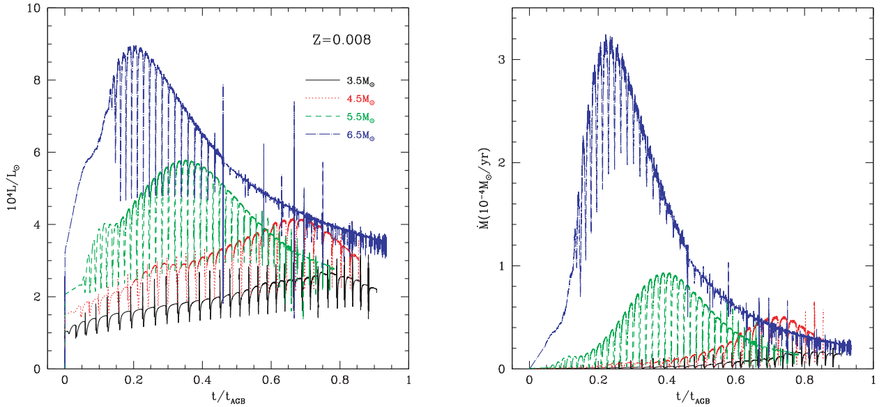
Figure 1. The variation of luminosity (left) and mass-loss rate (right) of models of different initial mass during the AGB phase. Times are normalized to the total duration of the AGB phase for each mass, indicated in Table 1. The various tracks refer to models of metallicity Z = 8 \times 10^{-3} and initial mass 3.5 M_\odot (black, solid track) 4.5 M_\odot (red, dotted), 5.5 M_\odot (green, dashed) and 6.5 M_\odot (blue, dot-dashed). [A colour version of this figure is available in the online version.]
