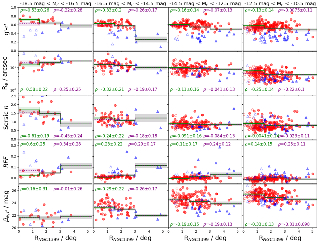
Fig. 15. Panel rows from top to bottom: g' - r' color, effective radius ( R_e ), Sérsic index ( n ), Residual Flux Fraction (RFF), and mean effective surface brightness ( \mu_{e,r} ) of the Fornax dwarf galaxies as a function of their cluster-centric distance. The columns correspond to different luminosity bins. The lines and shaded areas show the bin means and uncertainties of the mean for the parameters. The green and purple colors correspond to the values when the projection effects are taken in account (dE(nN)s and late-types excluded from the inner parts as found in Sect. 3.2), and when raw data is used, respectively. The late-type and early-type dwarfs are shown with the blue and red symbols, respectively. The unfilled symbols correspond to the galaxies excluded from the inner parts in order to minimize the projection bias. The \rho parameter indicates Spearman's correlation coefficient for the correlation of the parameter with distance, and its uncertainty.
