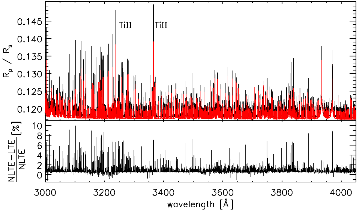
Fig. A.13. Same as Fig. 11, but for the 3000–4050 Å band.
