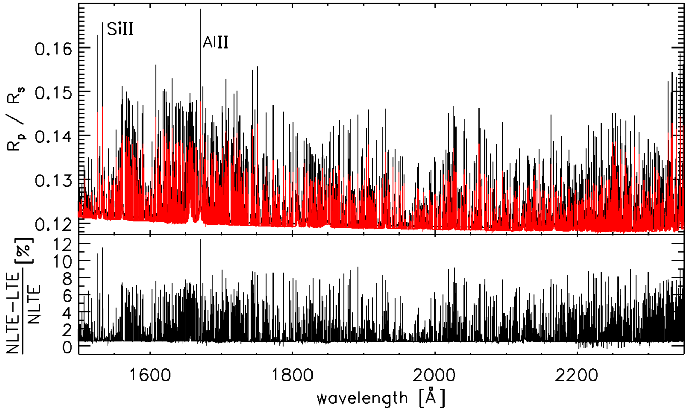
Fig. A.11. Same as Fig. 11, but for the 1500–2350 Å band.
