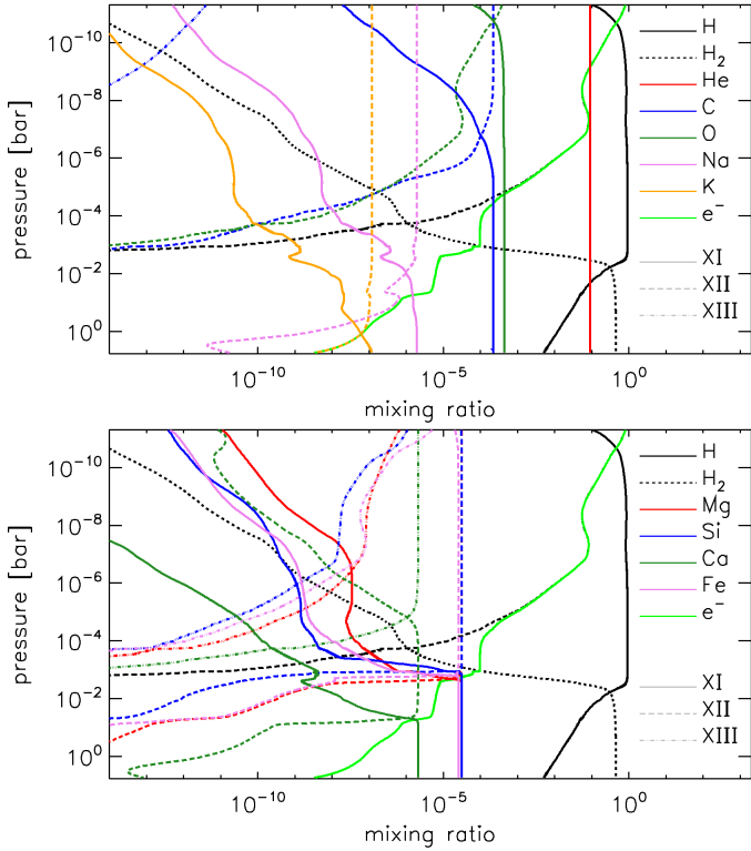
Fig. 4. Atmospheric mixing ratios obtained for metals. Top: mixing ratios for hydrogen (solid black line), H_2 (dotted black), He (red), C (blue), O (dark green), Na (violet), K (orange), and electrons (bright green) as a function of atmospheric pressure. Neutral (XI), singly ionised (XII), and doubly ionised (XIII) species are shown as solid, dashed, and dash-dotted lines, respectively. Bottom: same as the top panel, but for Mg (red), Si (blue), Ca (dark green), and Fe (violet). The hydrogen, H_2 , and e^- mixing ratios are shown in both panels for reference.
