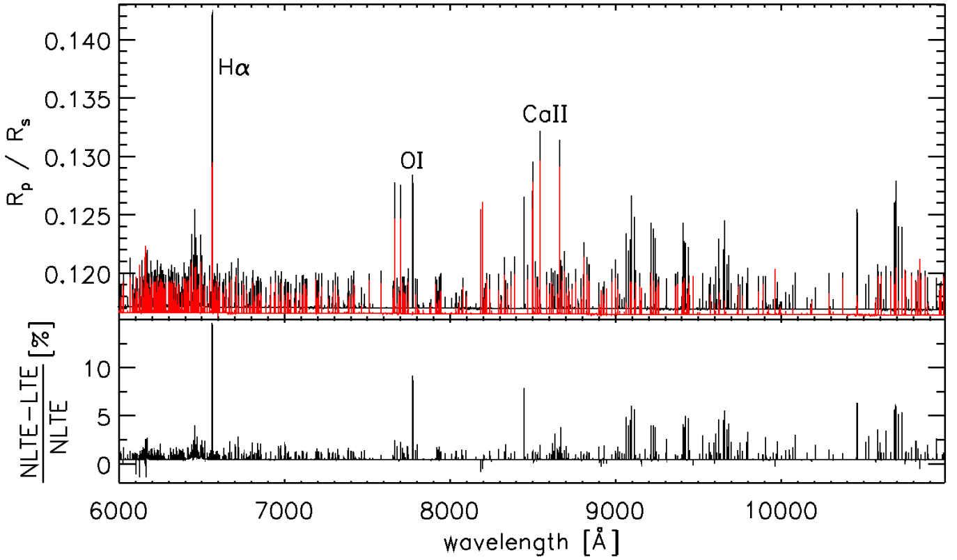
Fig. A.15. Same as Fig. 11, but for the 6000–11000 Å band.
