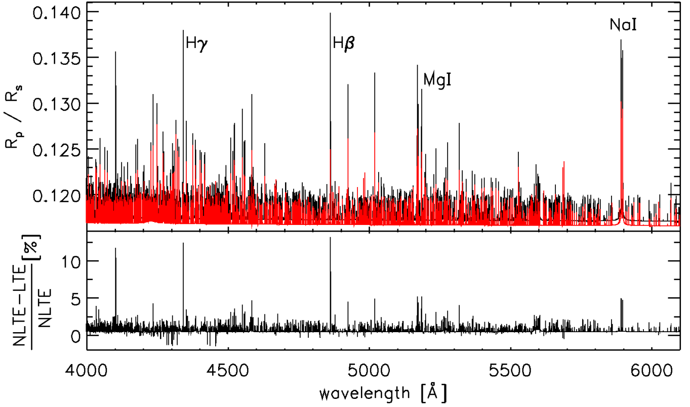
Fig. A.14. Same as Fig. 11, but for the 4000–6100 Å band.
