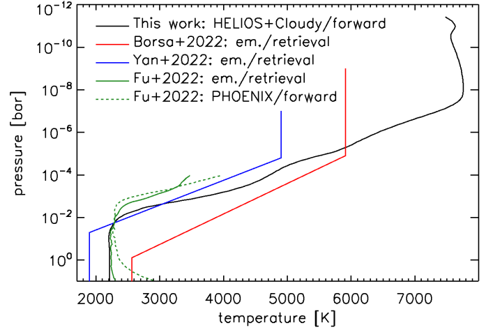
Fig. A.2. Comparison between our composite TP profile (black) with those published in the literature retrieved from secondary eclipse observations by Borsa et al. (2022) , Yan et al. (2022) , and Fu et al. (2022) , green). As a further comparison, the dashed green line shows the result of the forward model presented by Fu et al. (2022) . We recall that the retrieved profiles are an average over the illuminated planet disk; the black line is computed for the sub-stellar point.
