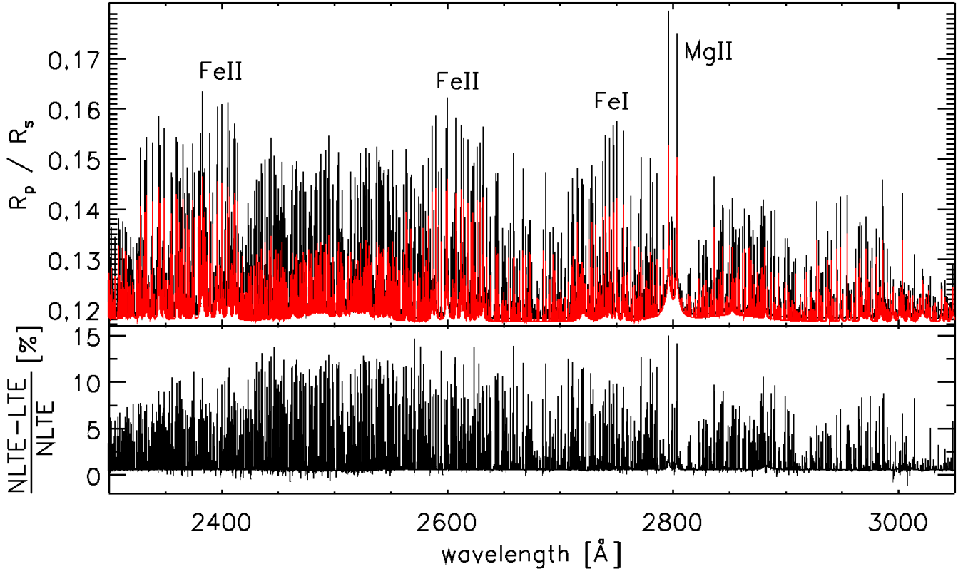
Fig. A.12. Same as Fig. 11, but for the 2300–3050 Å band.
