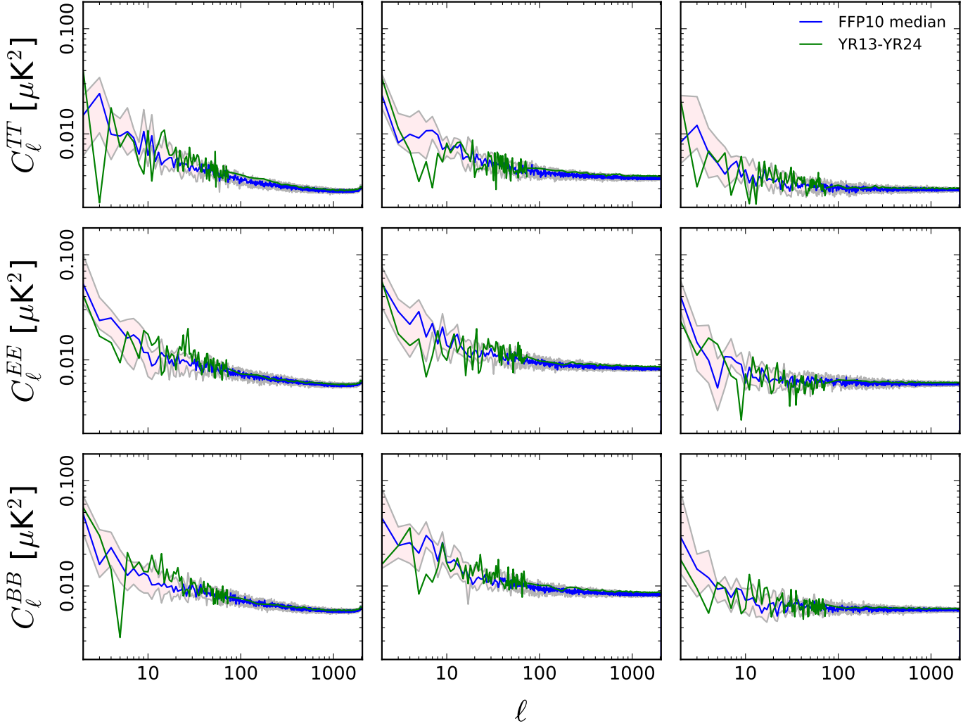
Fig. 24. Odd-even-year null spectra compared with simulations including the gain smoothing algorithm at 30 (left), 44 (middle), and 70 GHz (right). The pink band shows the 16 %–84 % quantile range of the simulations, with the median traced by the blue line. On large angular scales the data show larger variations with multipole than the simulations.
