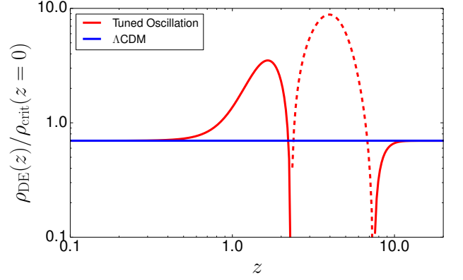
Figure 19. Implied variation in the energy density of the dark energy component for the model shown in Figure 18. The dotted line corresponds to the density becoming negative. These plots illustrate the difficulty of concurrently fitting the Ly \alpha and galaxy BAO constraints on D_M and D_H while satisfying the CMB constraint on D_M .
