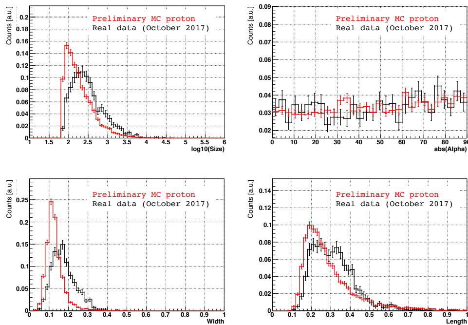
Figure 5. Normalized distributions of the main image parameters \log_{10}(\text{Size}) , Width, Length, and |\text{Alpha}| for the real proton shower events and the simulated ones (after the application of the same data reduction up to the image parameters calculation).
