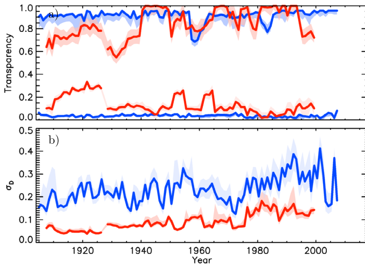
Figure 9 The maximum and the minimum values of transmittance ( top panel ) and the standard deviation of density values [ \sigma_D ] ( bottom panel ) within the solar disc for the DS1 ( red ) and DS2 ( blue ) data as a function of time. Shown are annual mean values ( solid lines ) along with the asymmetric 1 \sigma interval ( shaded surfaces ). These quantities are not defined for the Rome/PSPT data, which are given directly in units of intensity.
