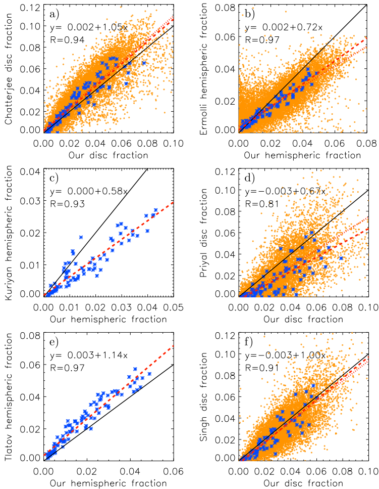
Figure 15 Plate areas presented in the literature (y-axis) versus the ones derived here from DS2 (x-axis): (a) Chatterjee, Banerjee, and Ravindra (2016) from DS2; (b) Ermolli et al. (2009b) from DS1; (c) Kuriyan, Muralidharan, and Sampath (1983) from the actual photographs; (d) Priyal et al. (2017) from DS2; (e) Tlatov, Pevtsov, and Singh (2009) from DS1; (f) Singh et al. (2018) from DS2. Blue asterisks (orange dots) show the annual (daily) values. The solid-black lines have a slope of unity. The dashed (dotted) red lines are linear fits to the annual (daily) data. Also shown are the corresponding parameters of the linear fits to the annual values and the linear correlation coefficients of the annual values.
