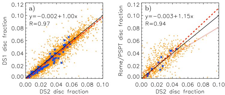
Figure 14 Scatter plots between the plage area values derived from images of DS2 (x-axis) and those from images (y-axis) of DS1 (panel a ) and Rome/PSPT (panel b ). Blue asterisks (orange dots) show the annual (daily) values. The solid black lines have a slope of unity and represent the expected value. The dashed (dotted) red lines are linear fits to the annual (daily) data. Also shown are the corresponding parameters of the linear fits to the annual values and the linear correlation coefficients of the annual values.
