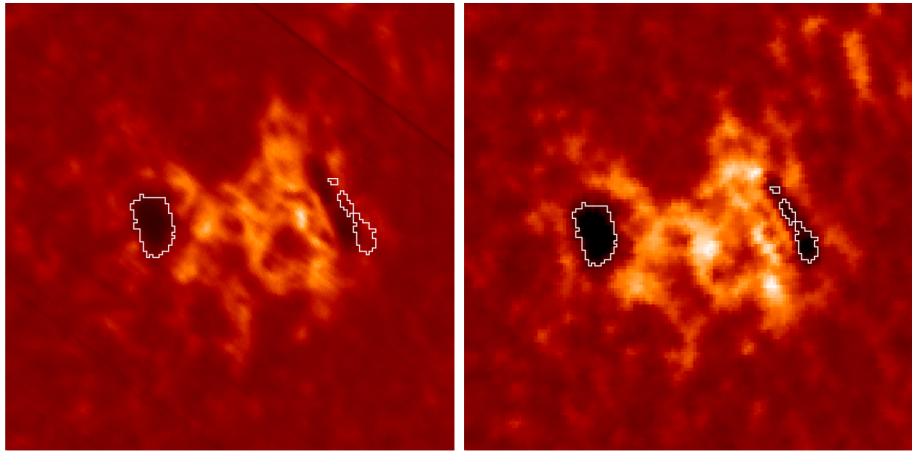
Figure 7 Enlargement of observations displayed in Figure 5 from DS2 (left) and Rome/PSPT (right) showing an active region. The images are saturated at [-0.5, 0.9] . The contours mark the location of sunspots as identified in the Rome/PSPT image. See Section 3.1 for more details. The spatial extent of each panel is roughly 268'' \times 268'' .
