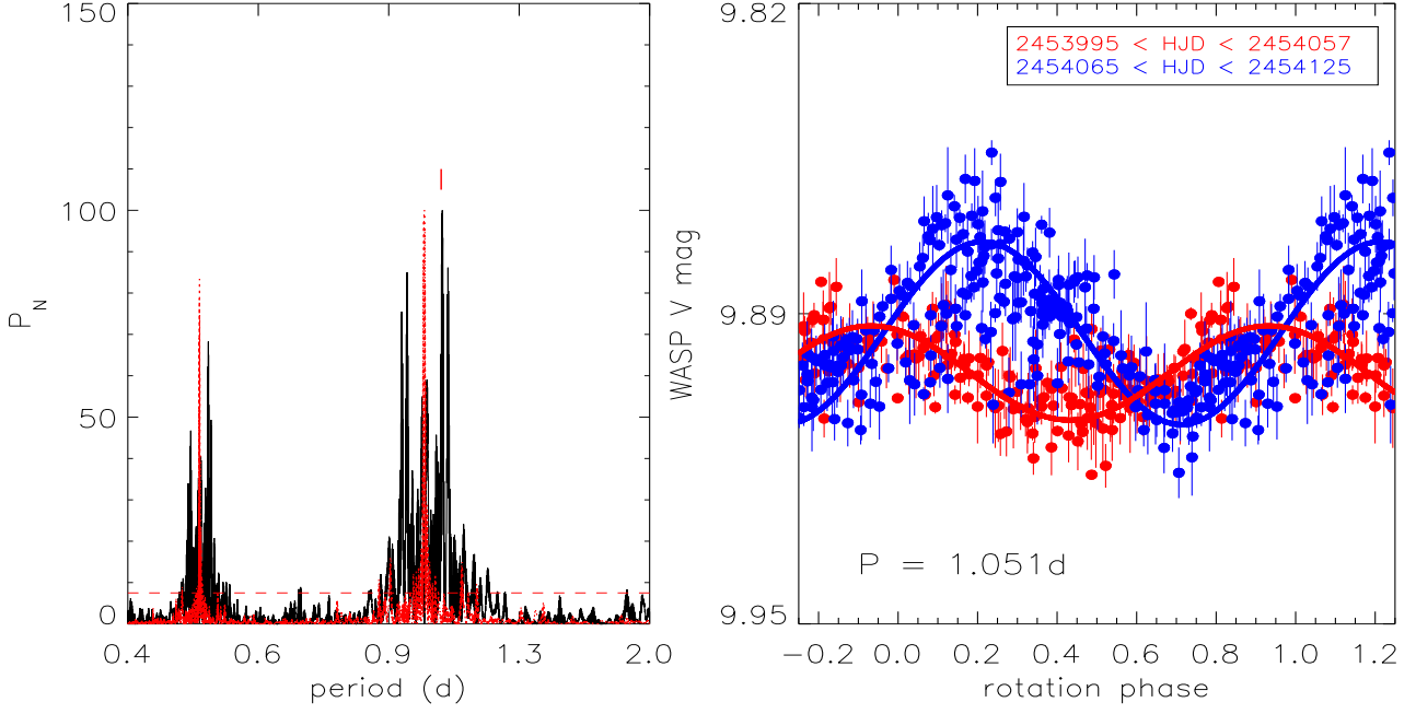
Fig. 5: Left panel: Lomb-Scargle periodogram of HD 284149 of the SuperWASP V magnitude time series collected in 2004 and 2006. The normalised power ( P_N ) (black solid line) is plotted versus period. The red dotted line represents the spectral window function, whereas the red horizontal dashed line indicates the power level corresponding to a FAP = 0.1%. Right panel: SuperWASP V magnitudes of HD 284149 collected in 2006 and phased with the photometric rotation period P = 1.051 \pm 0.005 days. Solid lines are the sinusoidal fits to phased data collected in the date range 2453995 < \text{HJD} < 2454057 (red) and in 2454065 < \text{HJD} < 2454125 (blue).
