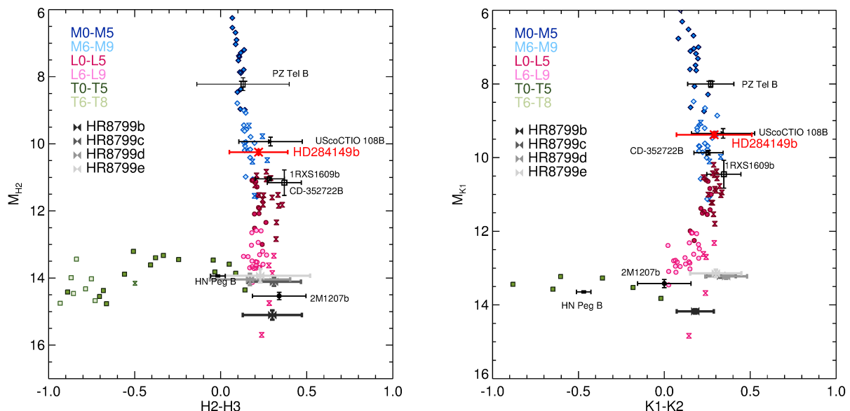
Fig. 13: Color–magnitude diagrams showing the position of HD 284149 b (red bow tie) relative to that of M, L and T field dwarfs and of young known companions, based on the H2-H3 photometry from the coronagraphic data (left panel) and the K1-K2 photometry from the non-coronagraphic data (right panel). See Section 4.1.1 for all the appropriate references and details on the construction of the plots.
