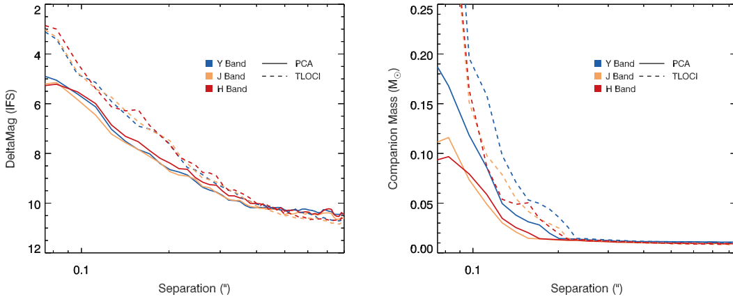
Fig. 2: IFS detection limits achieved during the non-coronagraphic observations of HD 284149 in terms of \Delta\text{mag} (left panel) and minimum companion mass (right panel) vs separation. The mass limits are evaluated using the COND models by Baraffe et al. (2003) and assuming an age of 35 Myrs. The different colours show the limits for the Y , J and H IFS filters respectively. The dashed line shows the limits evaluated using the images processed using the TLOCI method for speckle suppression (Marois et al. 2014), while the solid lines show the ones obtained using the images reduced using the PCA algorithm (Soummer et al. 2012; Amara & Quanz 2012).
