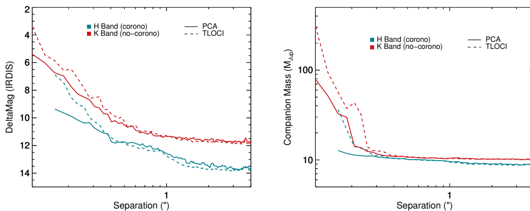
Fig. 3: IRDIS detection limits achieved during the observations of HD 284149 in terms of \Delta\text{mag} (left panel) and minimum companion mass (right panel) vs separation. The mass limits are evaluated using the BT-Settl models by Allard et al. (2012) and assuming an age of 35 Myrs. The blue and red curves show the limits achieved for the coronagraphic and non coronagraphic images, respectively. The dashed line shows the limits evaluated using the images processed using the TLOCI method for speckle suppression (Marois et al. 2014), while the solid lines show the ones obtained using the images reduced using the PCA algorithm (Soummer et al. 2012; Amara & Quanz 2012).
