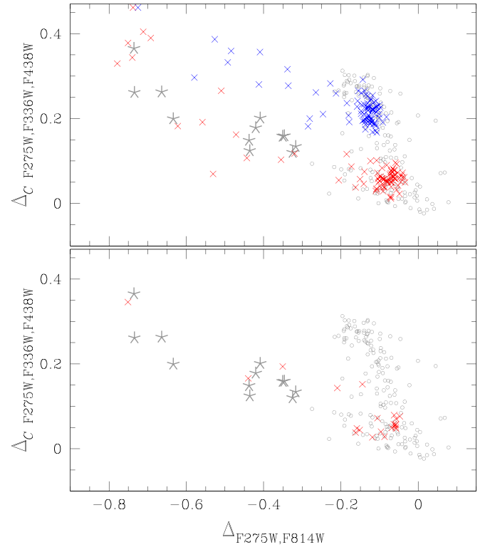
Figure 9. Observed ChM of NGC 3201 (gray symbols). The stars with extremely low \Delta_{F275W,F814W} are plotted as gray asterisks. Superimposed on the observed ChM are simulations of binary stars: in the top panel, we have simulated a cluster with 100% of the binaries, both 1G–1G (red) and 2G–2G (blue); in the bottom panel, we have simulated 12.8% of the binaries, which is the observed fraction on the main sequence (Milone et al. 2012b), by assuming that all of them are 1G–1G binaries.
