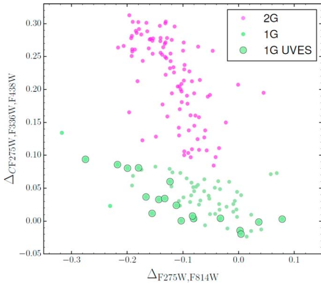
Figure 1. The ChM of NGC 3201 from Milone et al. (2017). Stars in green and magenta represent 1G and 2G stars, respectively, as defined by Milone and coworkers. Our 18 spectroscopic UVES targets are all located in the 1G region and highlighted as larger filled circles.
