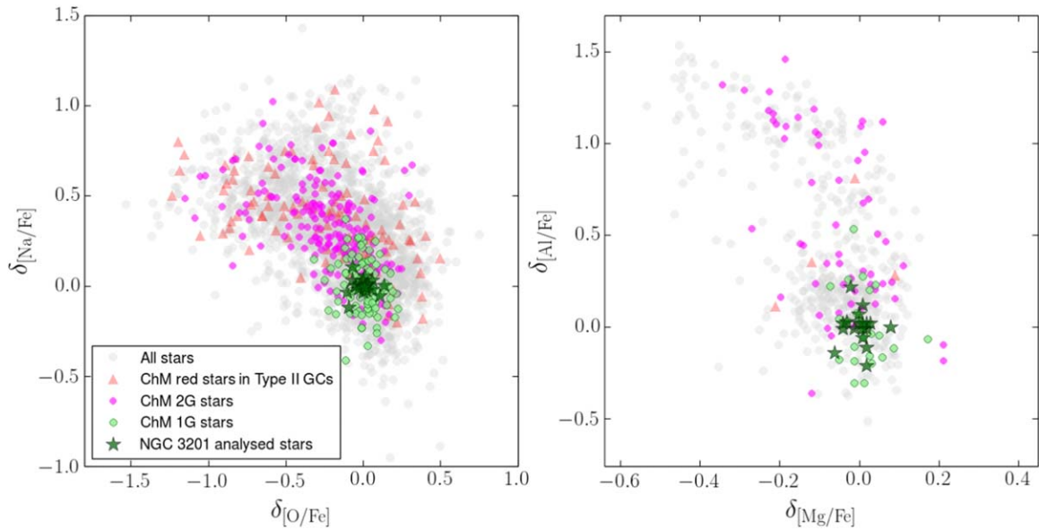
Figure 4. Abundance ratios of \delta_{[\text{Na}/\text{Fe}]} as a function of \delta_{[\text{O}/\text{Fe}]} (left) and \delta_{[\text{Al}/\text{Fe}]} as a function of \delta_{[\text{Mg}/\text{Fe}]} (right) for all GCs analyzed in Marino et al. (2019). The plotted abundances are relative to the average abundances of 1G stars, as defined by Marino and collaborators. Different symbols and colors represent stars belonging to different populations on the ChM. The abundances of the analyzed stars in NGC 3201 perfectly overlap with the ChM 1G abundances on these \delta_{[\text{O}/\text{Fe}]}-\delta_{[\text{Na}/\text{Fe}]} and \delta_{[\text{Mg}/\text{Fe}]}-\delta_{[\text{Al}/\text{Fe}]} planes.
