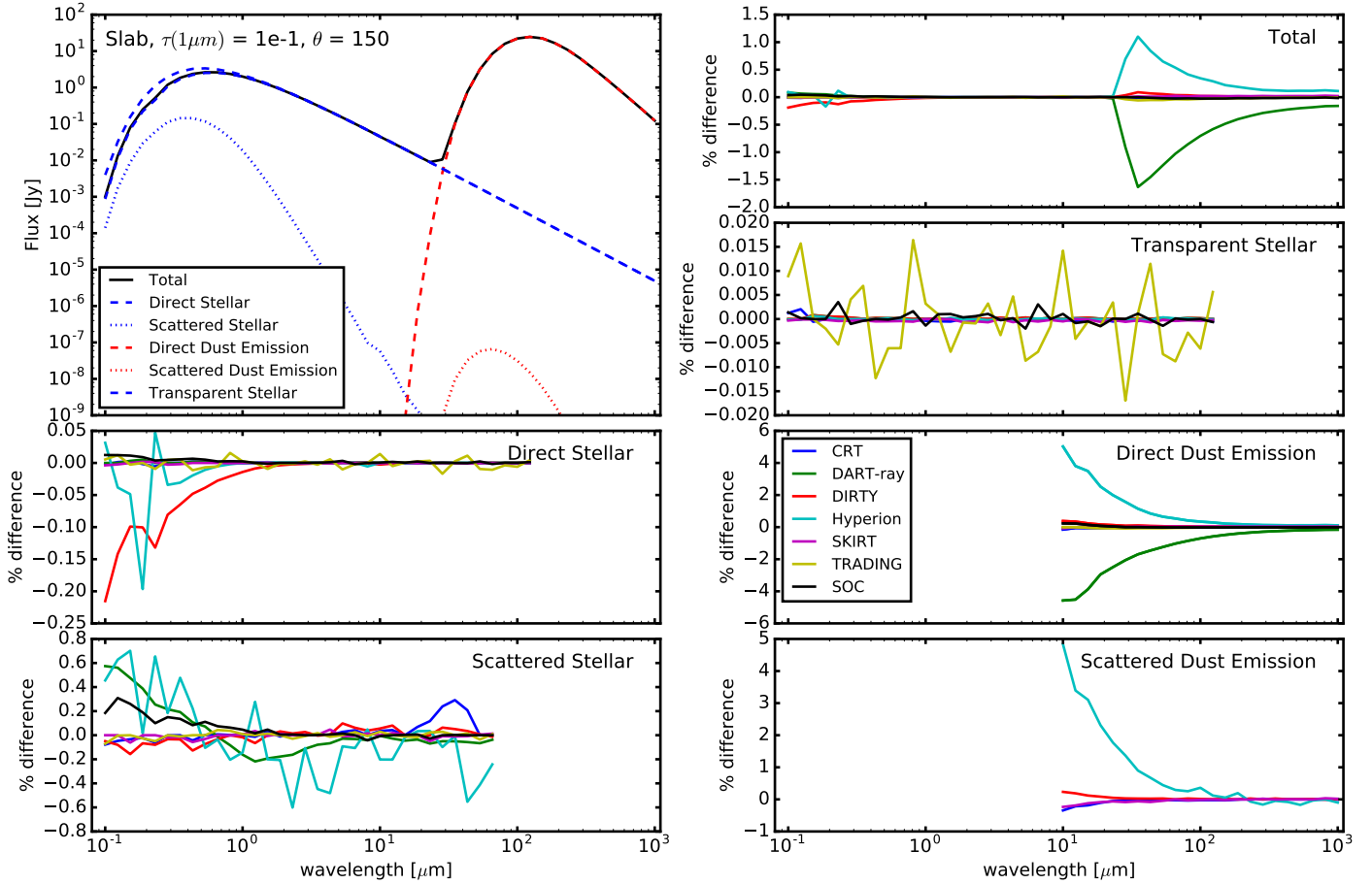
Fig. 6. An example of the model global SED outputs are shown for the \tau_z(1\ \mu\text{m}) = 0.1 , \theta = 150^\circ , and effective grain case. The plot in the upper left corner gives the median SED from all the models, both as a total and decomposed into components. The other plots give the percentage differences from the median for each of the components.
