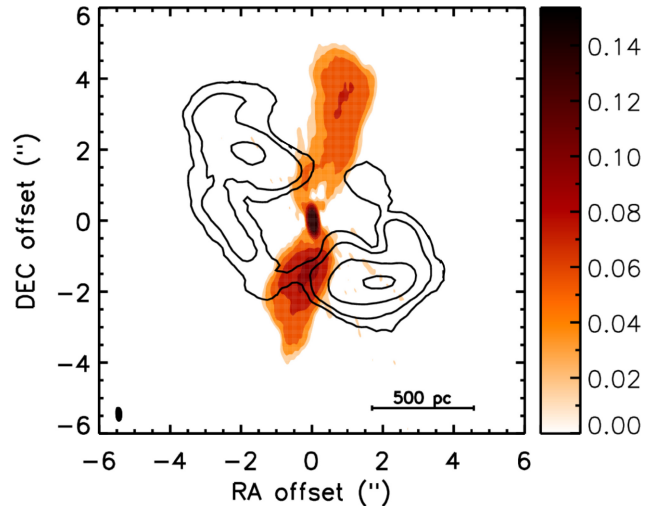
Figure 5. Masked JVLA continuum map of NGC 3100 at 10 GHz with ALMA CO(2–1) integrated intensity contours superimposed in black. CO contours are drawn at 9, 27, 81, and 180 times the 1\sigma rms noise level ( 1\sigma = 0.6 mJy beam ^{-1} ; see Paper I). The beam and the physical scale bars are drawn in the bottom-left and bottom-right corners, respectively. The wedge on the right shows the colour scale in Jy beam ^{-1} .
