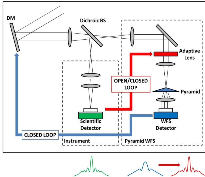
Figure 2: optical scheme of a possible astronomical instrument equipped with AO, with two channels: a scientific one, reaching the science detector (green), and a sensing one, reaching the P-WFS and the WFS detector (blue). After closing the loop, we obtain a high Strehl Ratio PSF (green) on the science path, while a degraded one (blue) on the sensing one. If a MAL (red) is inserted in the WFS channel, it allows to provide a high strehl PSF (red) also to the sensing channel and thus exploit the P-WFS characteristics. [PSF are just pictorial representations.]
