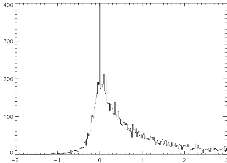
Figure 12: Count histogram obtained with a binning of 0.1. The different peaks (a,b,c,d) indicate regions on the map where the flux is uniform. The corresponding contours are identified on the map of W44.
